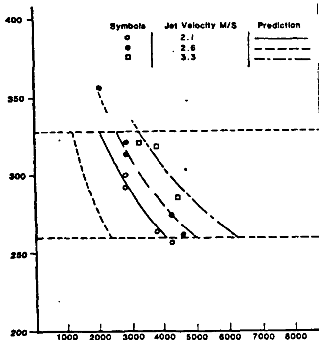
Figure 6 Operation range for the 150\text{ }\mu\text{m} orifice size plate.
