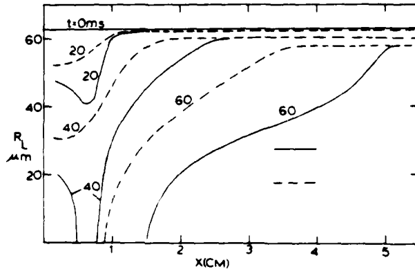
Fig. 9 Droplet Radius Profiles, With and Without Droplet Ignition
