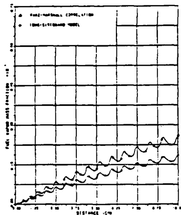
FIG. 12 FUEL VAPOR MASS FRACTION VERSUS DISTANCE AT 16 MILLISECONDS FOR DIFFERENT GAS-PHASE MODELS
