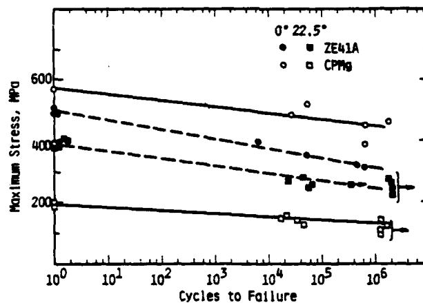
Fig. 2—Effect of fiber orientation and matrix alloy addition on the fatigue behavior of \text{Al}_2\text{O}_3 fiber-reinforced magnesium.
