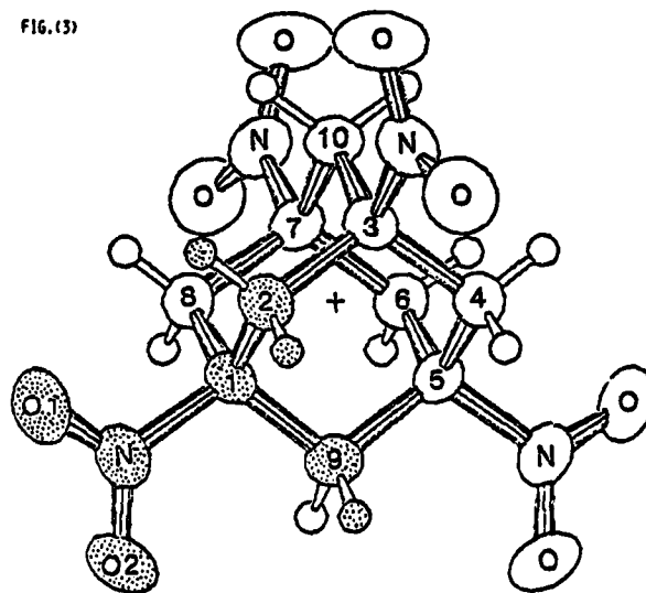
1,3,5,7-TETRANITROADAMANTANE
