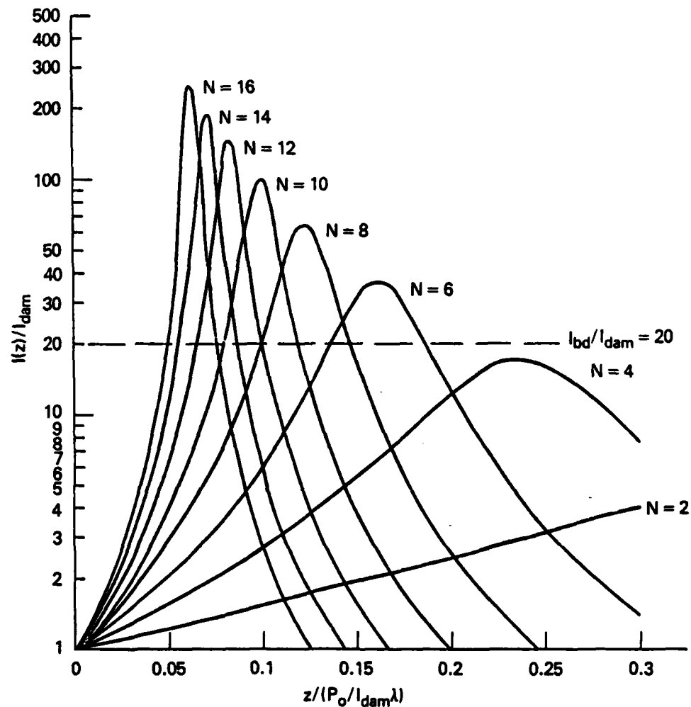
Figure 9. Plot of the intensity along the optical axis of a focussed Gaussian beam for various values of Fresnel number. The intensity is normalized to the intensity at the lens, and the axial position is normalized to a number that is related to focal length. The breakdown threshold is also shown.
