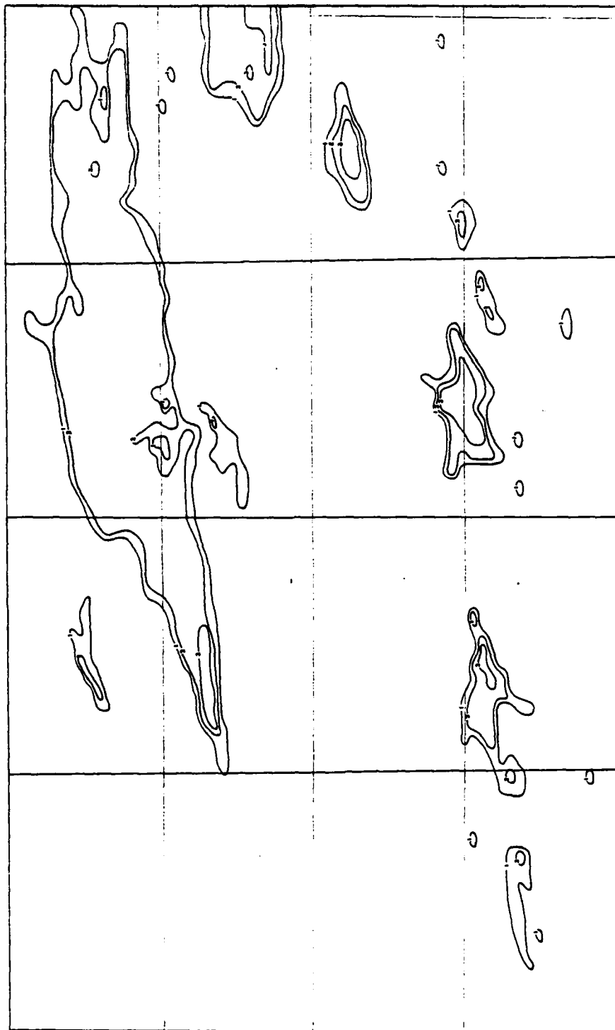
Figure 22. SPADS Contoured Precipitation Intensity for 11 AUG 83
