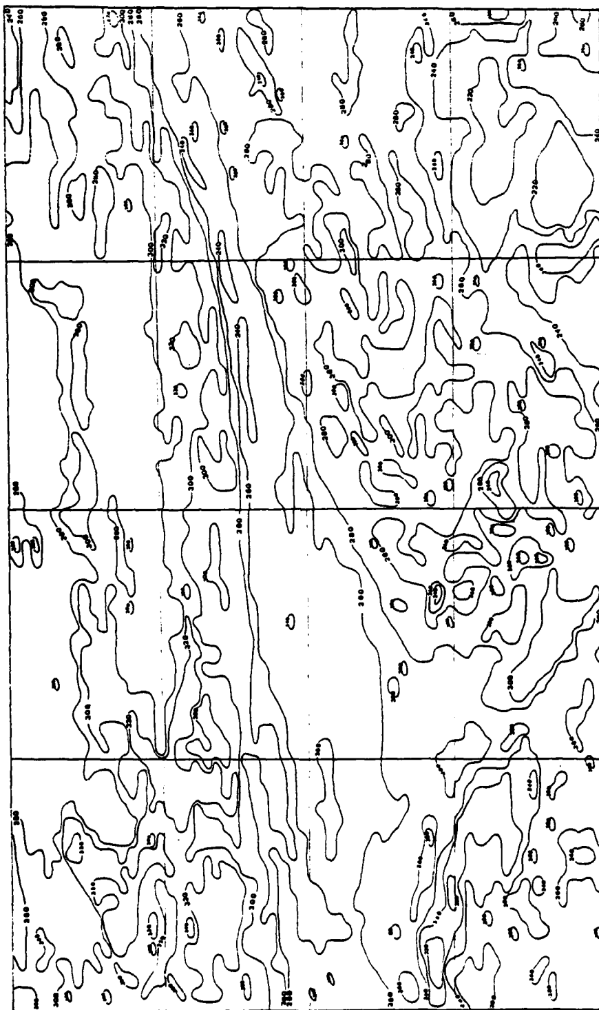
Figure 14. SPADS Contoured Cloud-Top Temperature for 02 AUG 83
