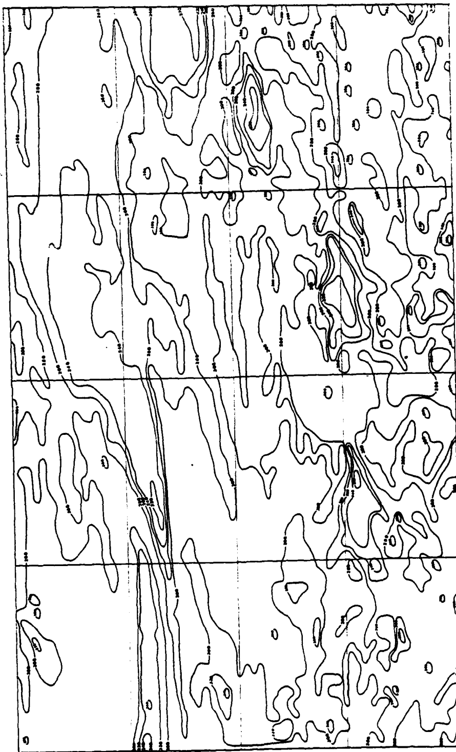
Figure 23. SPADS Contoured Cloud-Top Temperature for 11 AUG 83
