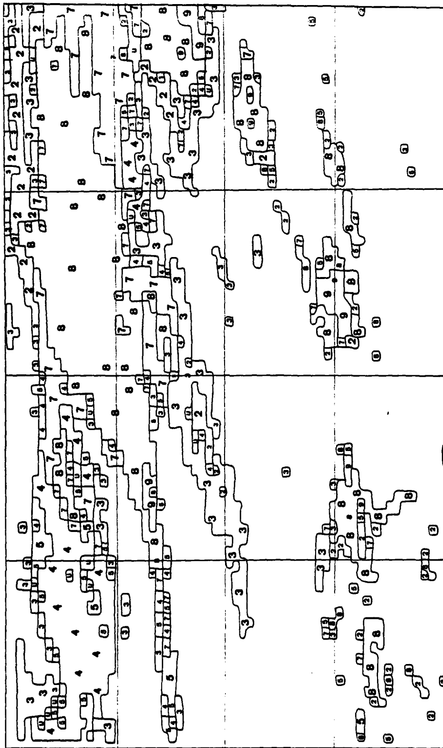
Figure 21. SPADS Contoured Cloud Type for 11 AUG 83
