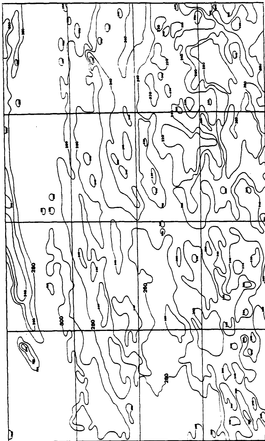
Figure 50. SPADS Contoured Cloud-Top Temperature for 02 SEP 83
