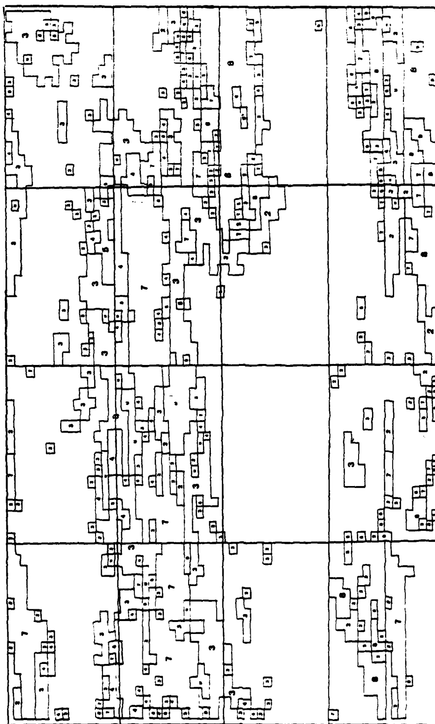
Figure 30. SPADS Contoured Cloud Type for 23 AUG 83
