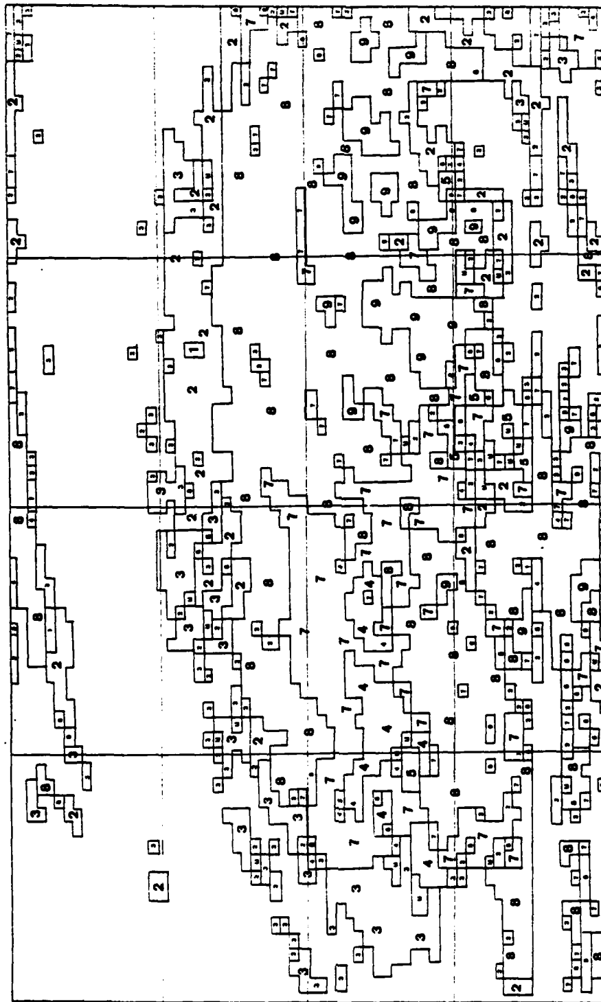
Figure 47. SPADS Contoured Cloud Type for 02 SEP 83
