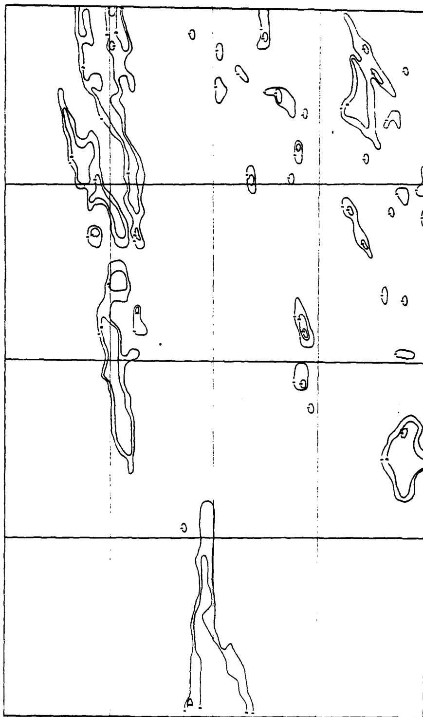
Figure 40. SPADS Contoured Precipitation Intensity for 31 AUG 83
