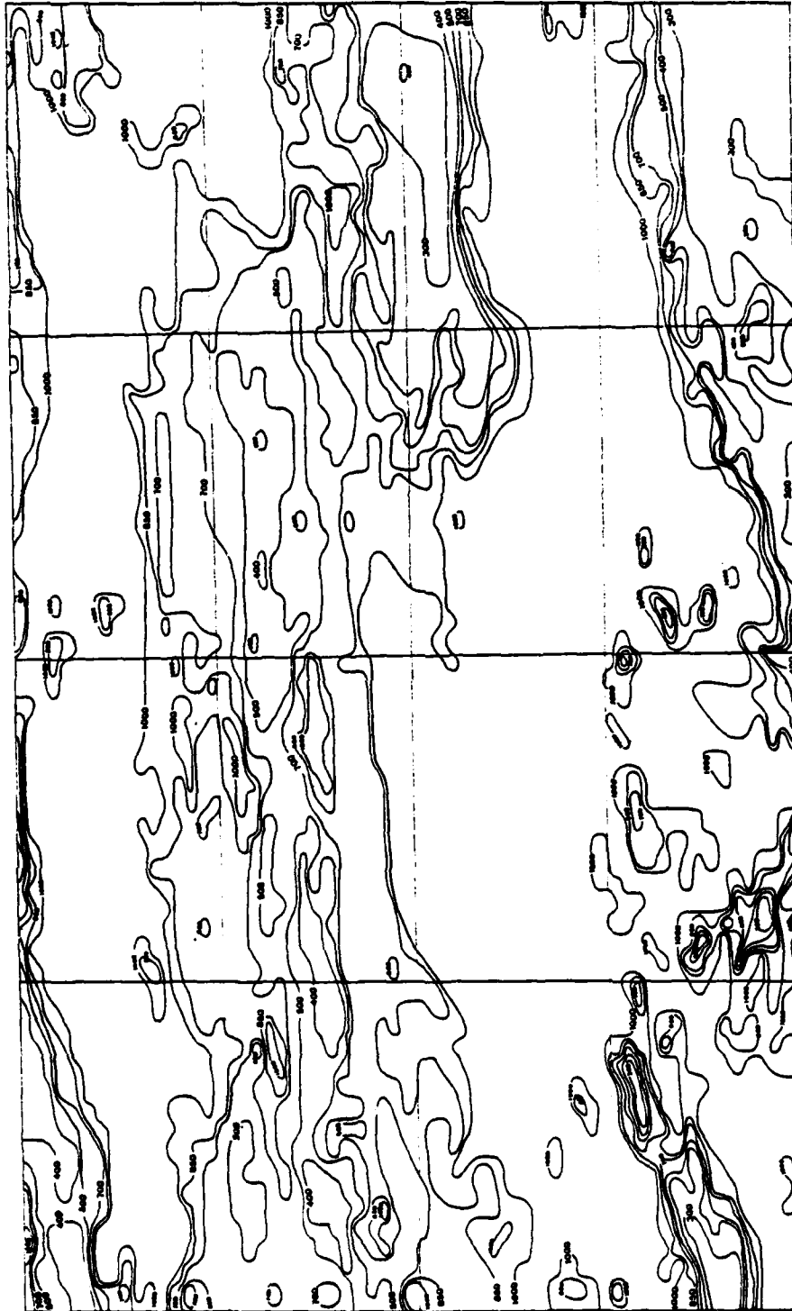
Figure 33. SPADS Contoured Cloud-Top Height for 23 AUG 83
