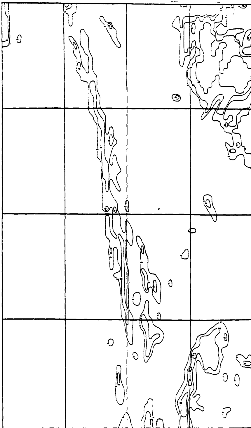
Figure 13. SPADS Contoured Precipitation Intensity for 02 AUG 83
