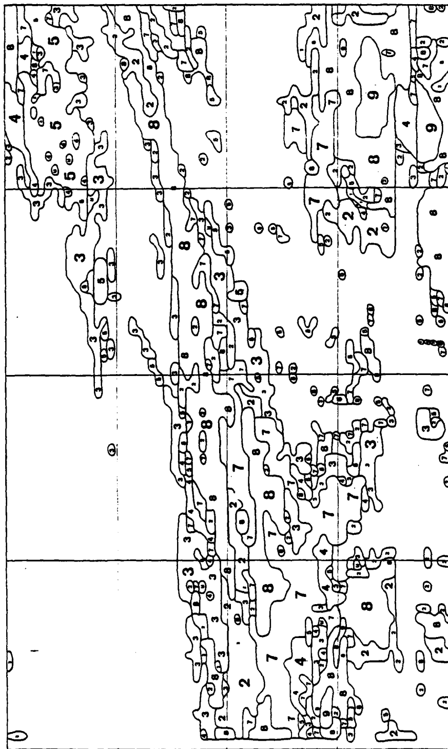
Figure 12. SPADS Contoured Cloud Type for 02 AUG 83
