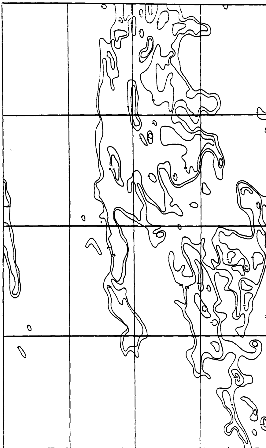
Figure 49. SPADS Contoured Precipitation Intensity for 02 SEP 83
