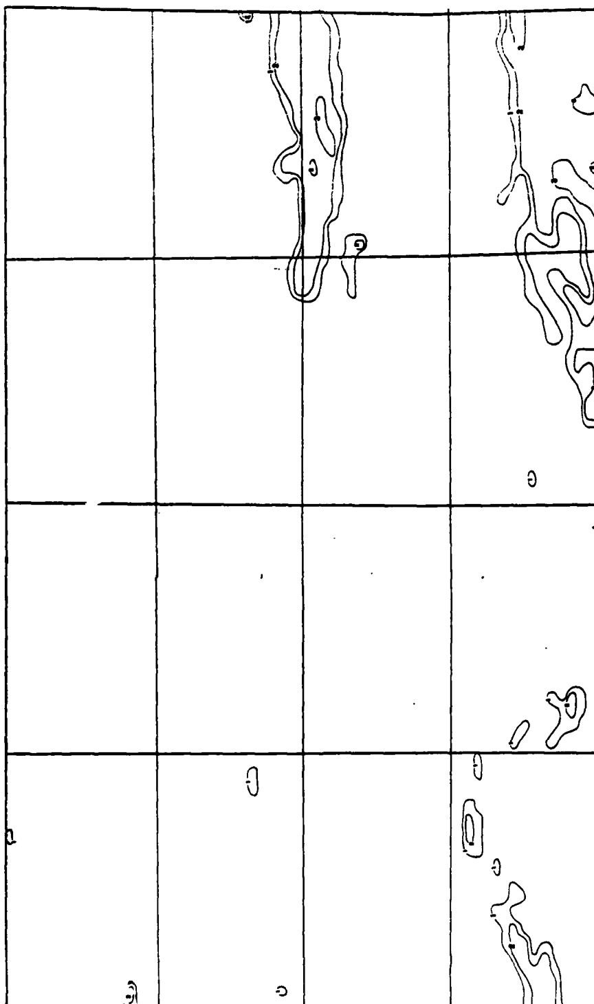
Figure 31. SPADS Contoured Precipitation Intensity for 23 AUG 83
