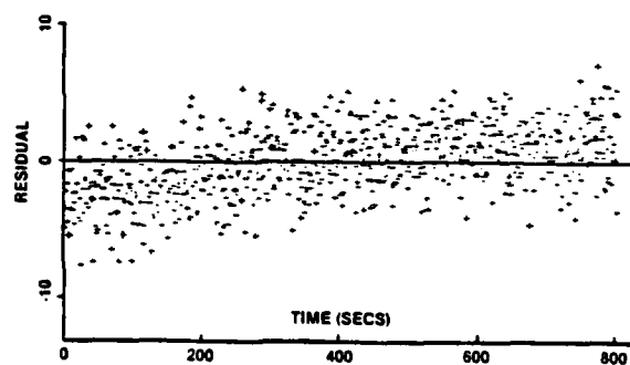
Figure 10. Bearing Residual vs Time; \theta=\theta_5 , R/R_{true}=2.4 , S/S_{true}=1.0
