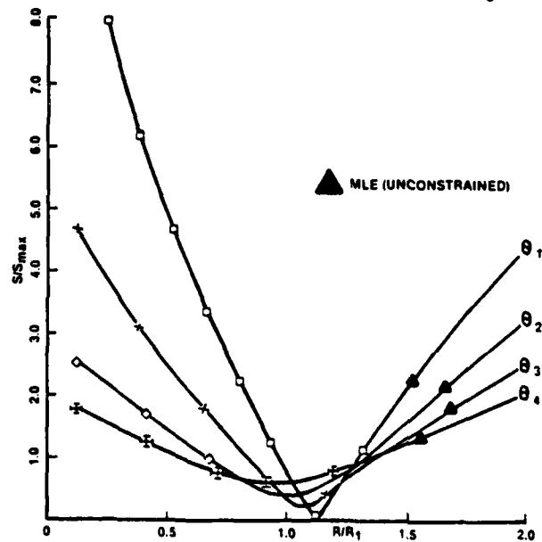
Figure 6. Observed Dynamic Behavior in Constrained Estimation: Normalized Speed vs Normalized Range Constraint
