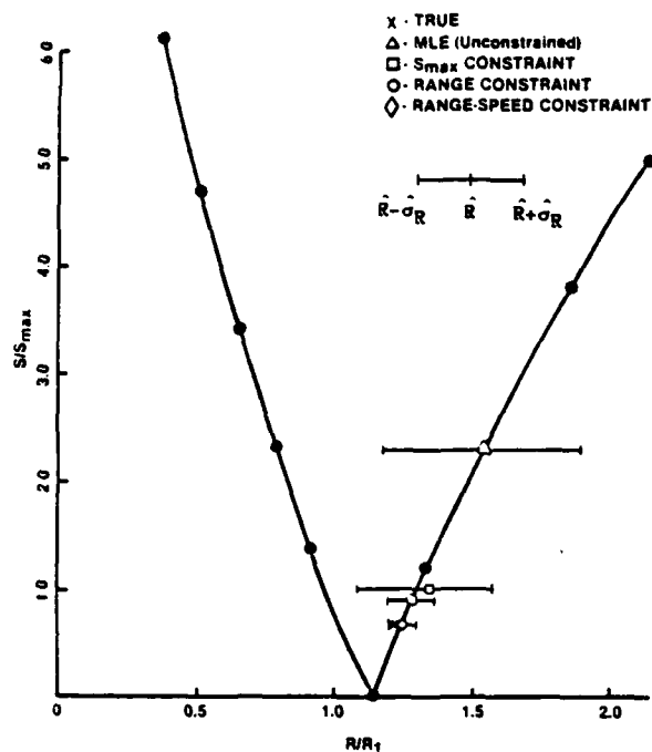
Figure 11. Solution Enhancement via Utilization of Heuristic Information ( \theta = \theta_1 )
