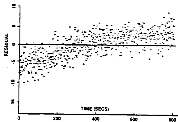
Figure 13b. Bearing Residual vs Time; \theta = \theta_6 , R/R_{true} = 2.3 , S = S_{max}
