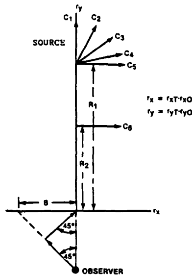
Figure 1. Source-Observer Geometries
