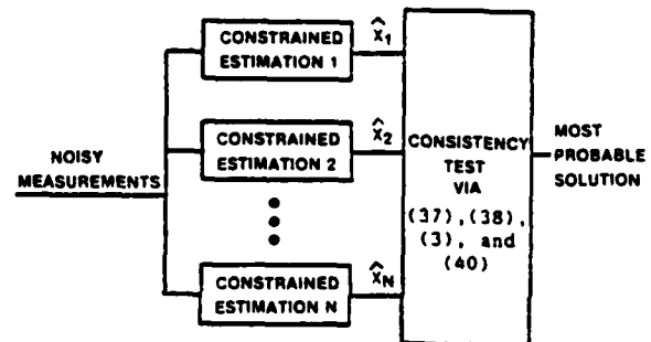
Figure 5. Estimation Configuration with Limited A Priori Information (Multiply-Connected Region)
