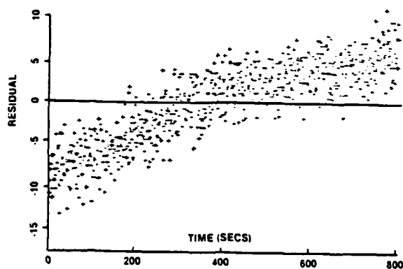
Figure 13c. Bearing Residual vs Time; \theta = \theta_6 , R/R_{true} = 3.4 , S = S_{max}
