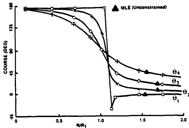
Figure 7. Observed Dynamic Behavior in Constrained Estimation: Course vs Normalized Range Constraint
