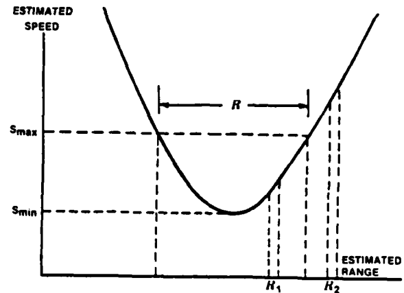
Figure 4. Potential Application of Constrained Estimation: Solution Selection
