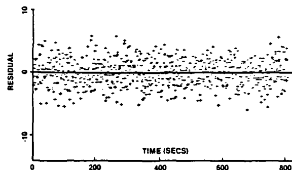
Figure 13a. Bearing Residual vs Time; \theta = \theta_6 , R/R_{true} = 1.0 , S = S_{true} < S_{max}
