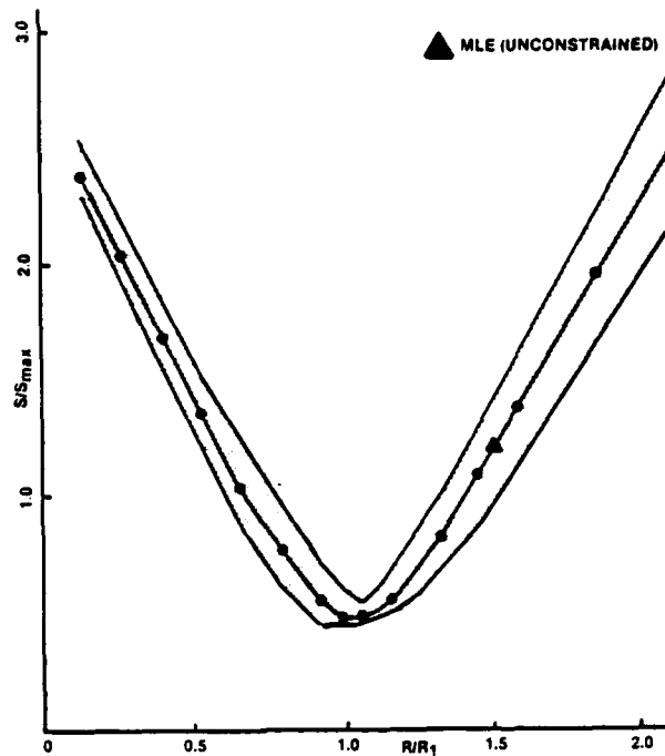
Figure 9. Region of Minimal \sigma_{\beta}^2
