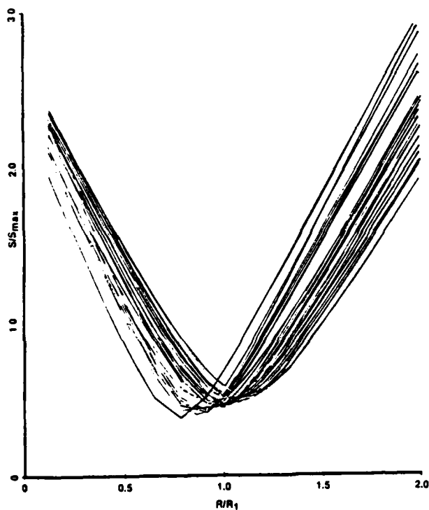
Figure 8. Normalized Speed vs Normalized Range Constraint ( 0=\theta_5 ) for 30 Noise Sequences
