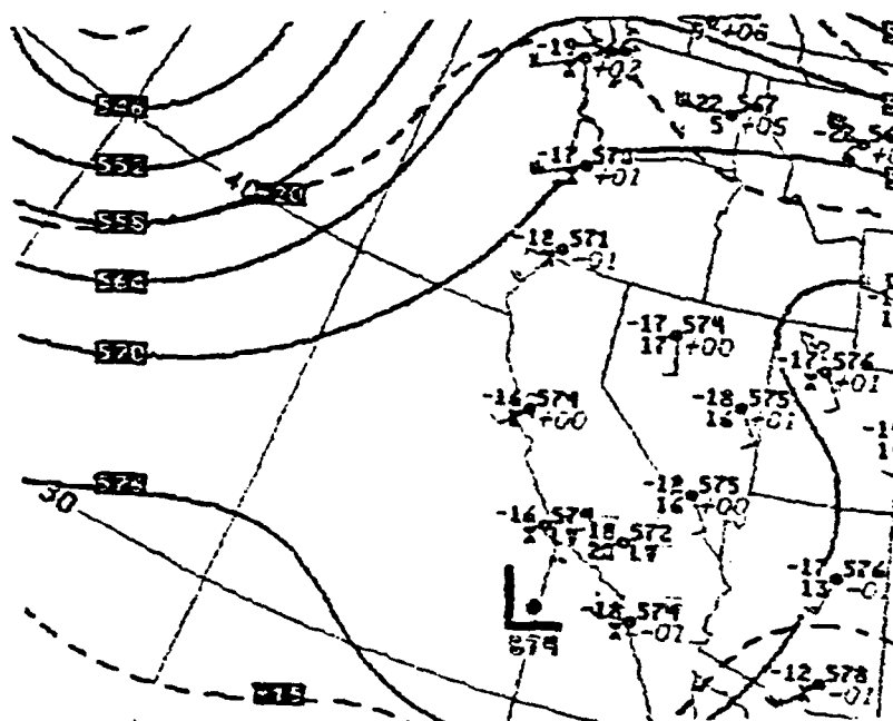
Figure 3.15 Surface (a) and 500 mb (b) analyses 1200 GMT 14 April 1977.
