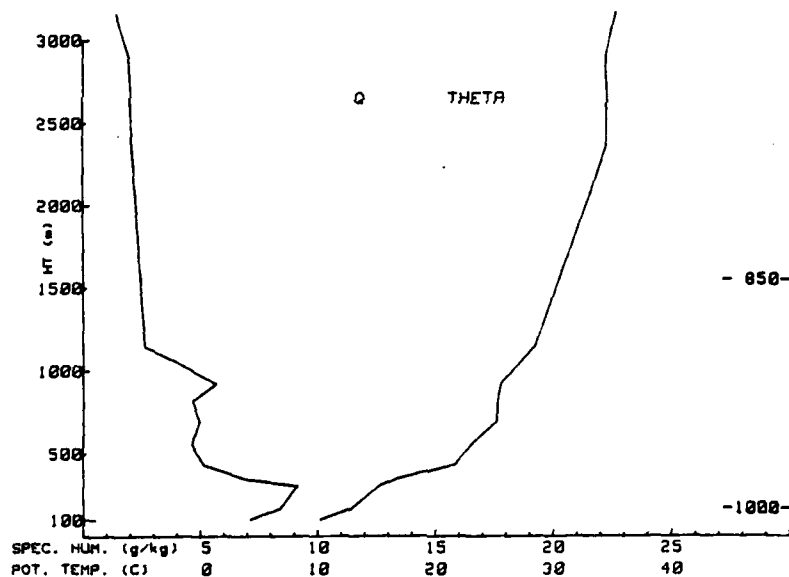
Figure 3.8 Example of Winter Case rawinsonde.
