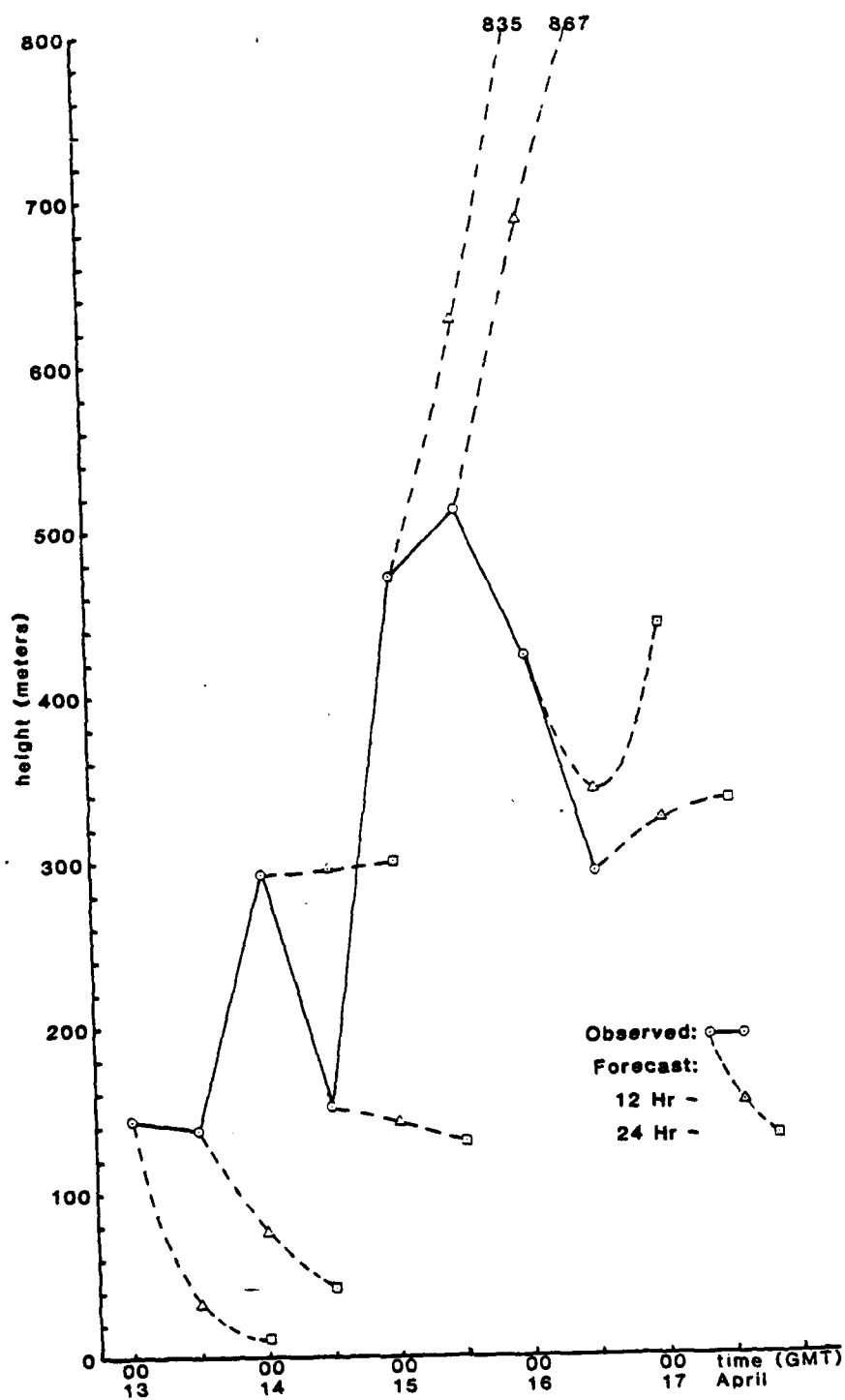
Figure 4.3 Graphical Depiction of Spring Case Observed and Forecasted Inversion Heights.
