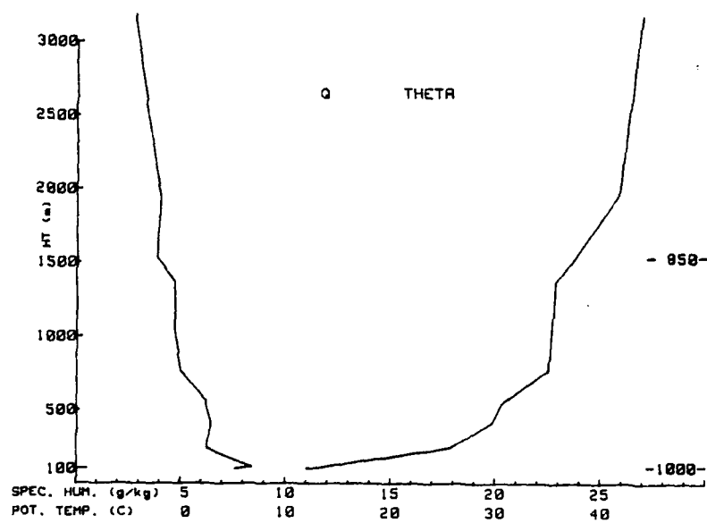
(b) 1200 GMT Sounding
