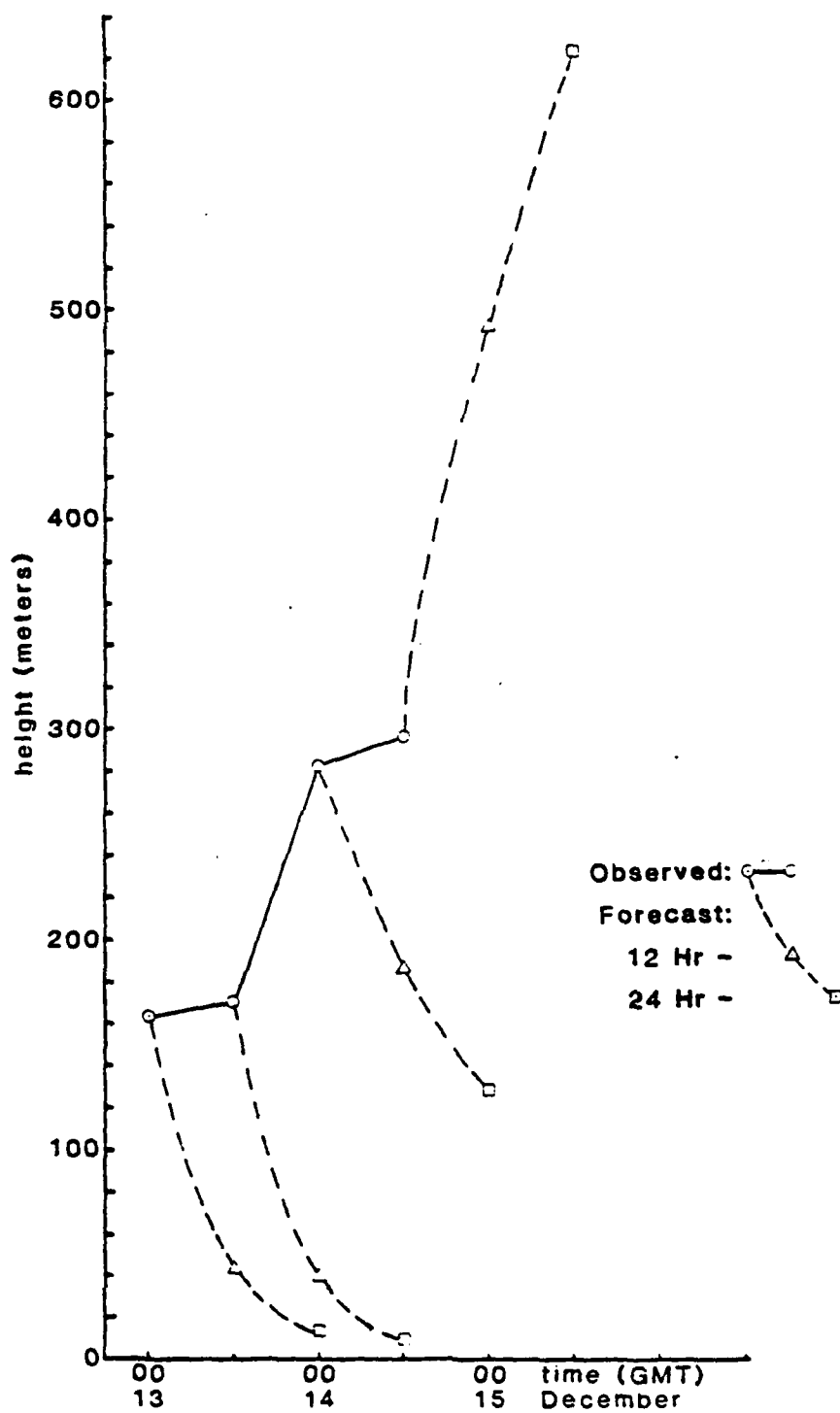
Figure 4.2 Graphical Depiction of Winter Case Observed and Forecasted Inversion Heights.
