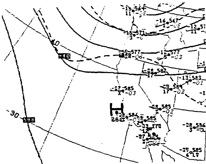
Figure 3.29 Surface (a) and 500 mb (b) analyses 1200 GMT 4 September 1977.
