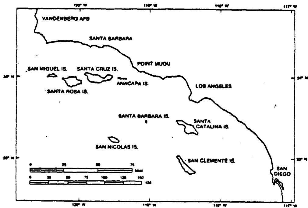
Figure 1.1 Southern California Coastal Regions.
