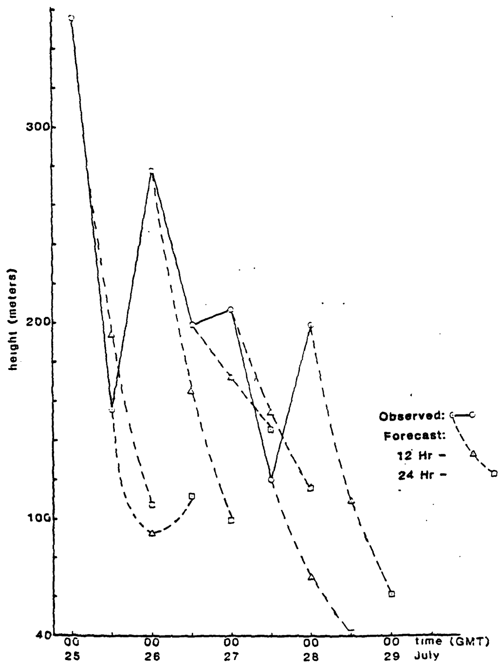
Figure 4.1 Graphical Depiction of Summer Case Observed and Forecasted Inversion Heights.
