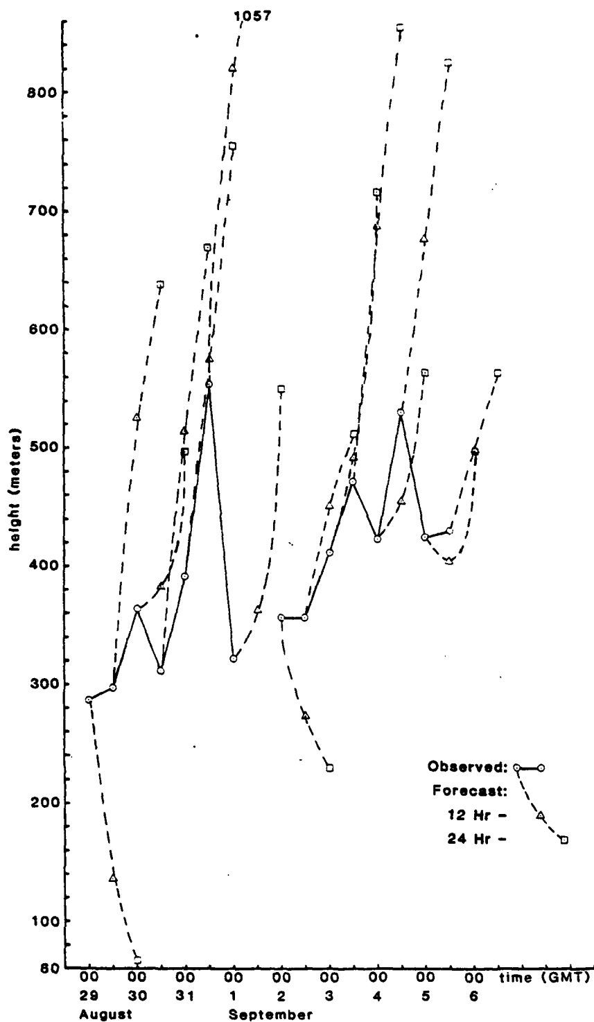
Figure 4.4 Graphical Depiction of Fall Case Observed and Forecasted Inversion Heights.
