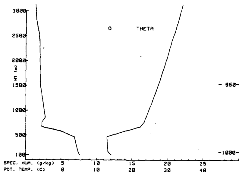
Figure 3.13 Example of rawinsonde for Spring Case.
