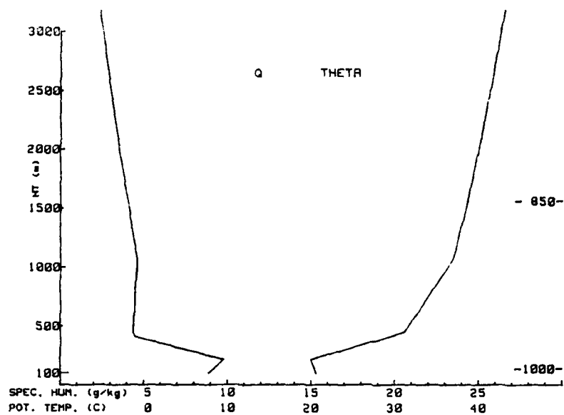
(a) 0000 GMT Sounding
