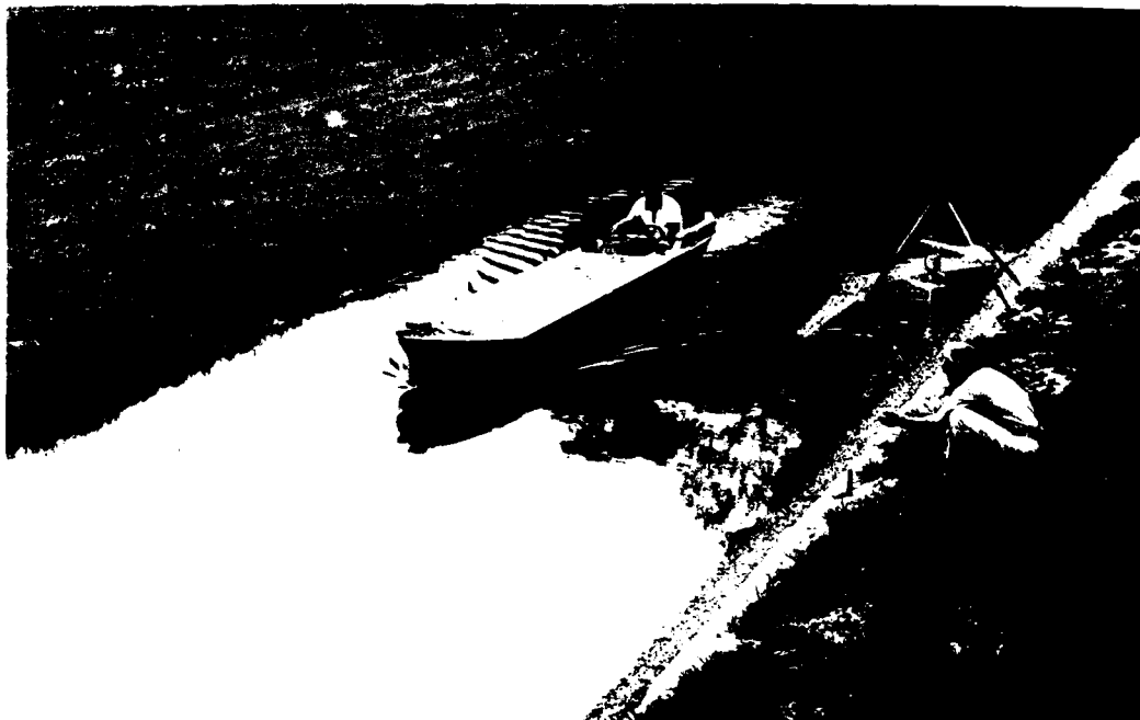
Figure I-2. 1:30-scale ship in SRDWSC model
