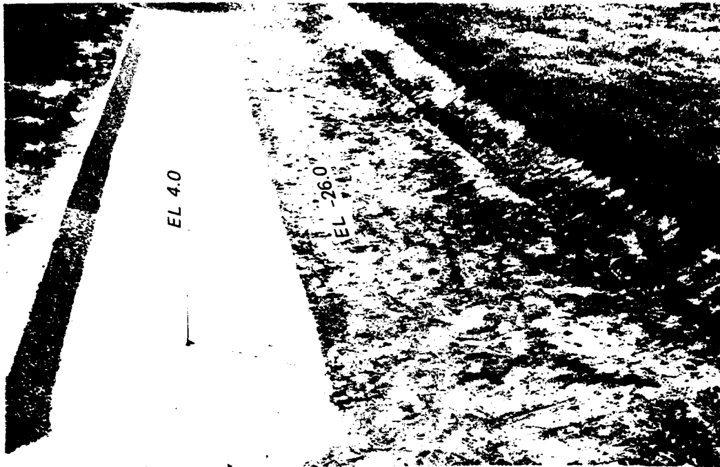
Figure I-1. 1:30-scale model of 0.5-mile reach of SRDWSC
