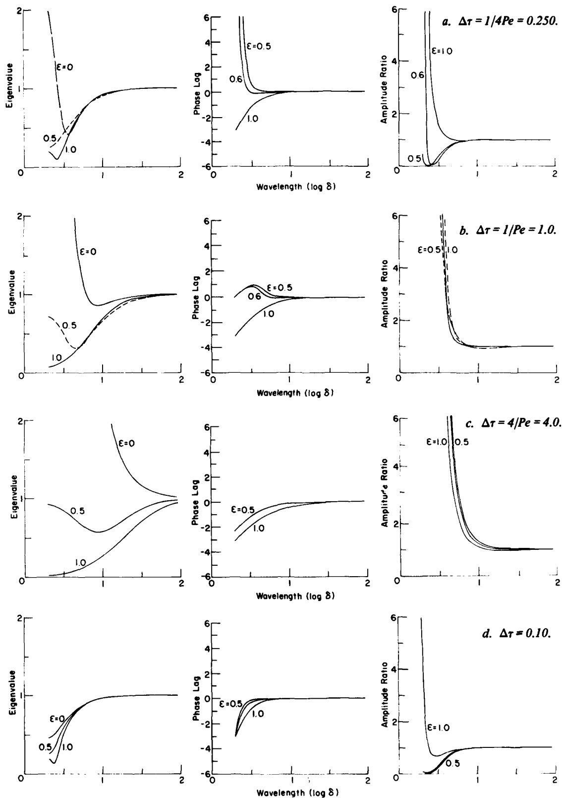
Figure 50. Eigenvalue, phase lag and amplitude ratio vs wavelength when Pe = 1.0 . The abscissa is the base ten logarithm of the nondimensional wavelength \delta .
