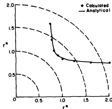
Figure 26. Comparison of the two-phase corner results with the analytical solution.
