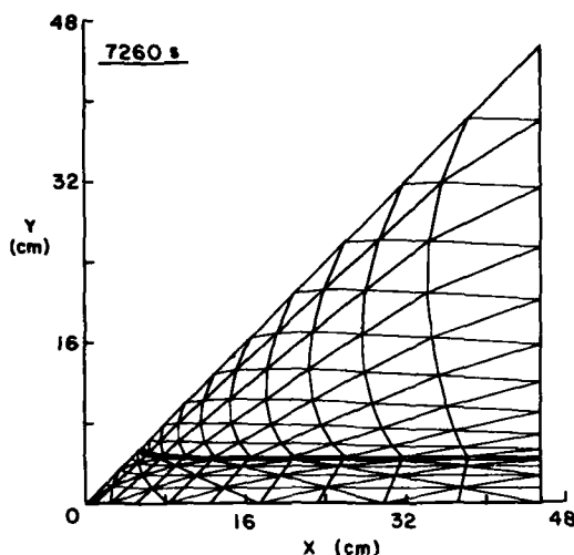
Figure 24. Final mesh for the two-phase corner comparison.
