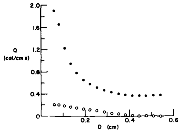
Figure 45. Heat flow Q vs ice thickness D at the end of the 5-m pipe when freeze-up occurs. The closed circles represent flux from the ice; the open circles represent flux from the water.
