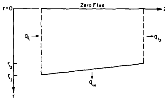
Figure 36. Heat flow into and out of an increment of fluid.
