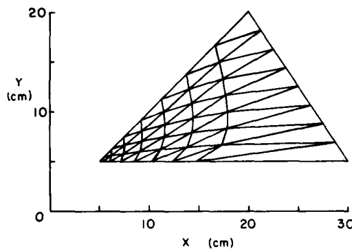
Figure 8. Use of the trilinear projector, using uneven divisions along the sides.
