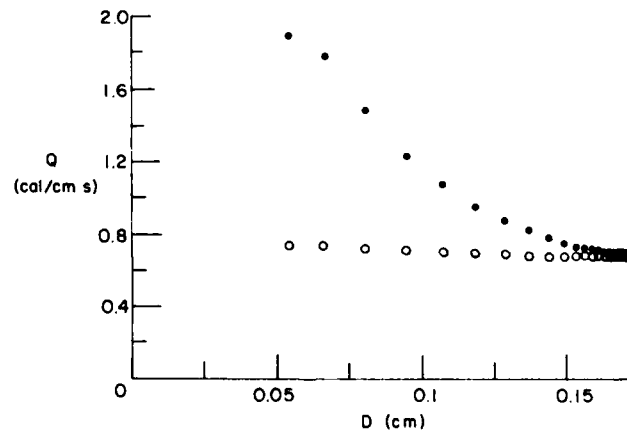
Figure 42. Heat flux Q vs ice thickness D at the end of the 1-m pipe, where the ice profile achieved a steady state. The closed circles represent flux from the ice; the open circles represent flux from the water.
