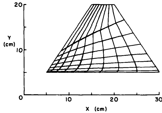
Figure 7. Use of the bilinear projector with method 2, using uneven divisions along the sides.
