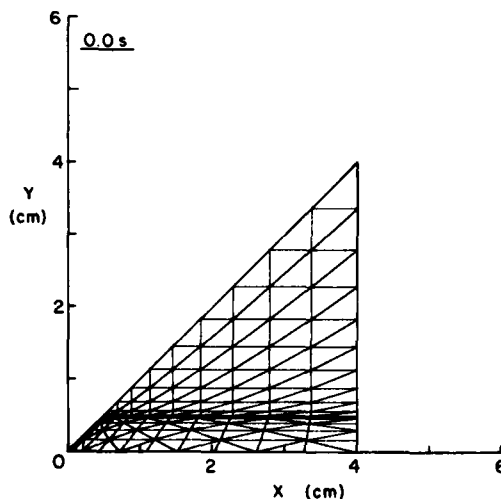
Figure 22. Initial mesh for the two-phase corner comparison.
