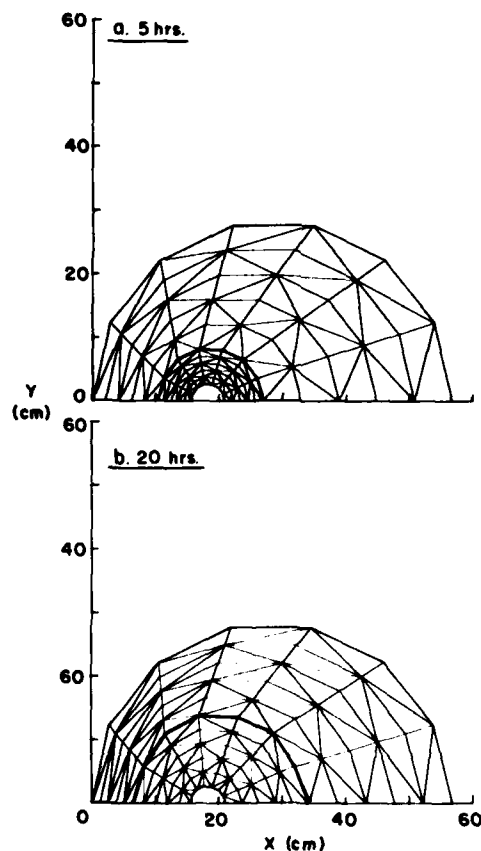
Figure 32. The mesh for the experiment comparison (case 1). The phase front is highlighted for clarity.
