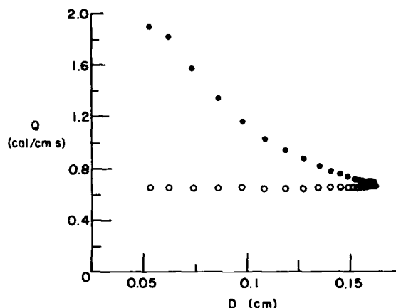
Figure 48. Heat flux Q vs ice thickness D for the 5-m pipe where a steady state flow occurs. The closed circles represent flux from the ice; the open circles represent flux from the water.
