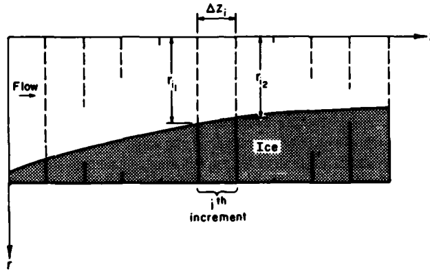
Figure 35. Schematic diagram of pipe with ice interface.
