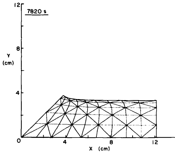
Figure 19. Final mesh for the one-phase corner problem.
