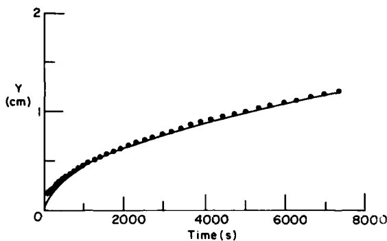
Figure 14. Phase front location comparison with the one-phase Neumann solution. The solid line is the analytical solution; the circles represent the calculated solution.
