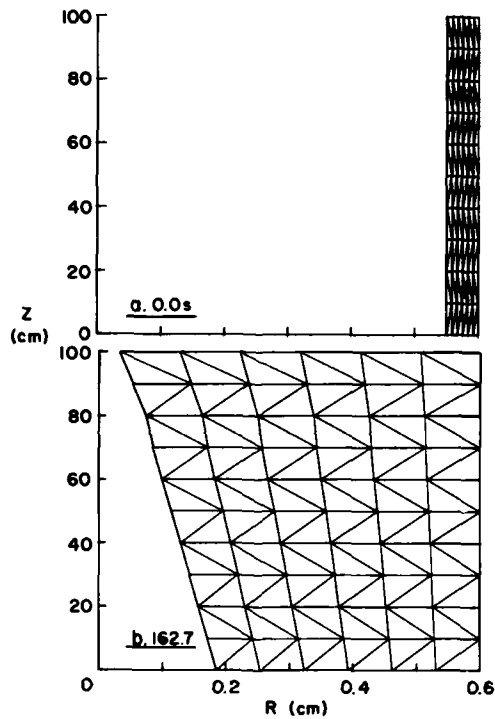
Figure 37. Initial mesh and mesh just before freeze-up for the 1-m pipe.
