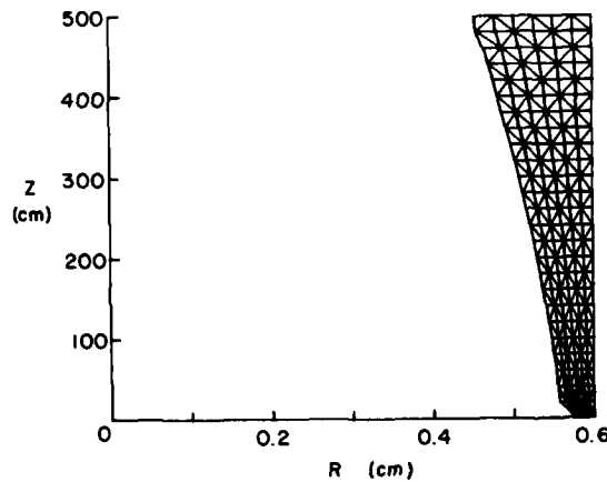
Figure 46. Final mesh for the 5-m pipe, a steady-state ice profile.
