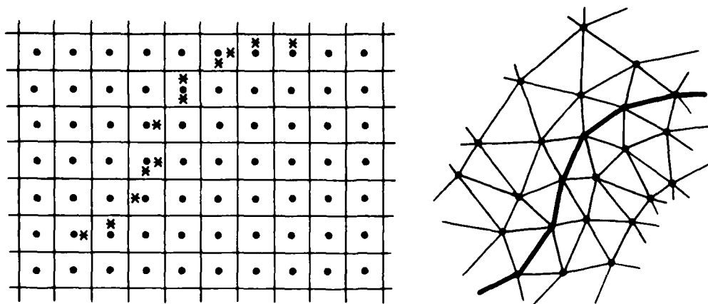
a. Use of apparent heat capacity method with finite differences. Solid dots represent nodes, and stars represent the interpolated location of the phase front.
