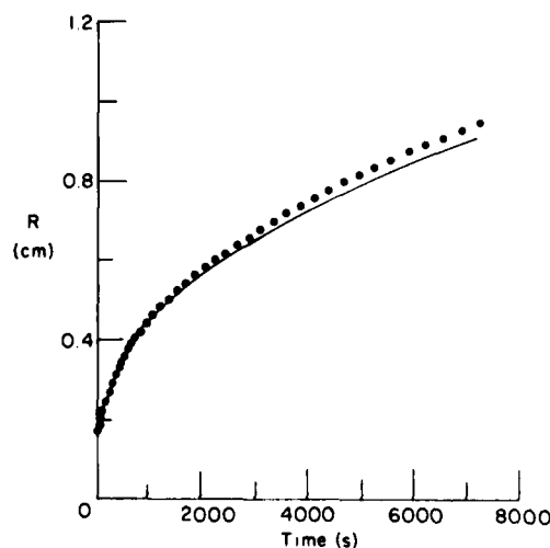
Figure 16. Phase front location comparison with the quasi-steady radial solution. The solid line is the analytical solution; the circles represent the calculated solution.
