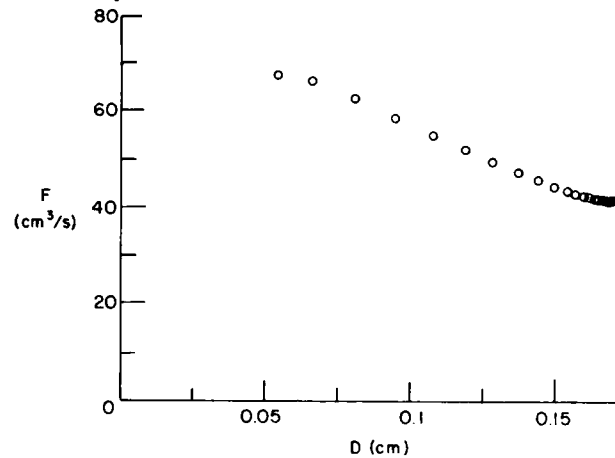
Figure 41. Flow rate F vs ice thickness D at the end of the 1-m pipe, where the ice profile achieved a steady state.
