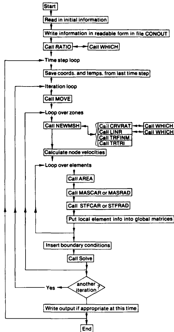
Figure 13. Flow chart for Femove.
