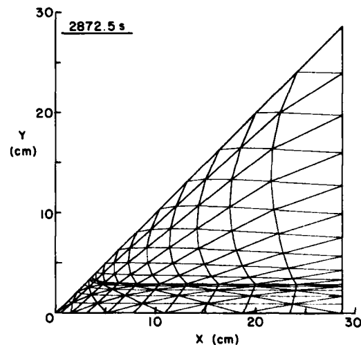
Figure 23. The mesh at an intermediate time step.
