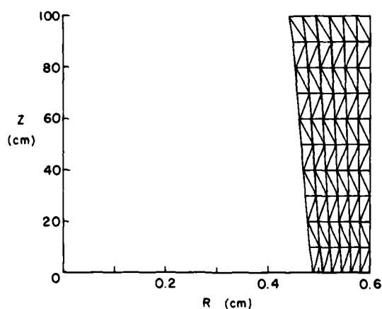
Figure 40. Final mesh, a steady-state ice profile.
