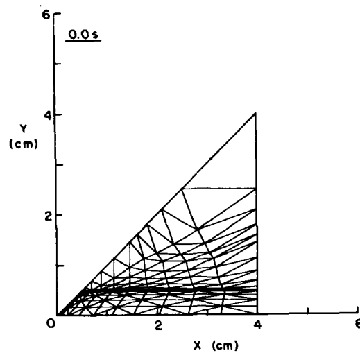
Figure 27. Initial mesh for two-phase corner problem where numerical distortion of the temperature solution occurred.
