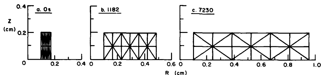
Figure 17. Initial, intermediate and final meshes for the radial comparison.
