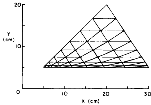
Figure 9. Use of the trilinear projector, using uneven but proportional side divisions.
