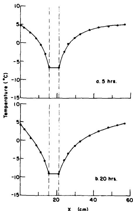
Figure 31. Temperature comparison along horizontal axis of symmetry for case 1. The dots represent data from the experiment. The solid line represents the numerical solution. The dashed lines represent the pipe.
