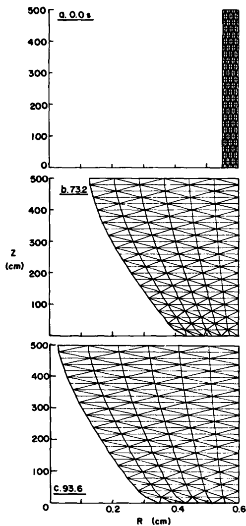
Figure 43. Initial mesh, intermediate mesh, and mesh just before freeze-up for the 5-m pipe.
