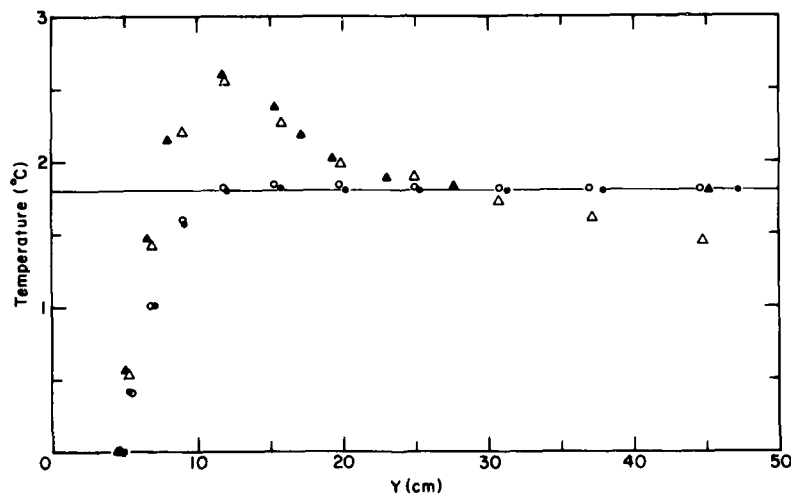
Figure 28. Temperatures at nodes along the vertical zero-flux boundary in the unfrozen zone:
