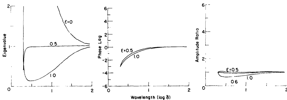
Figure 49. Eigenvalue, phase lag and amplitude ratio vs wavelength when Pe = 80 . The abscissa is the base ten logarithm of the nondimensional wavelength \delta .
