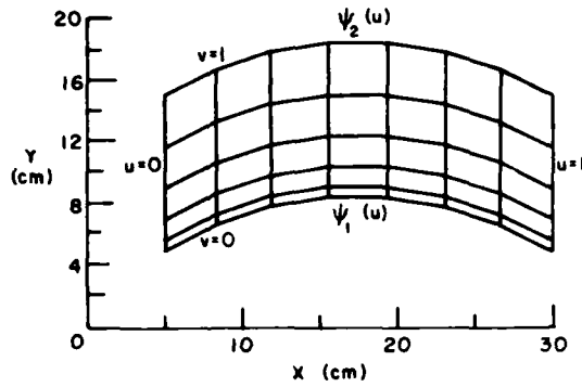
Figure 3. Use of the lofting projector.
