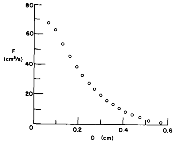
Figure 38. Flow rate F vs ice thickness D at the end of the 1-m pipe, in the case where the pipe freezes up.
