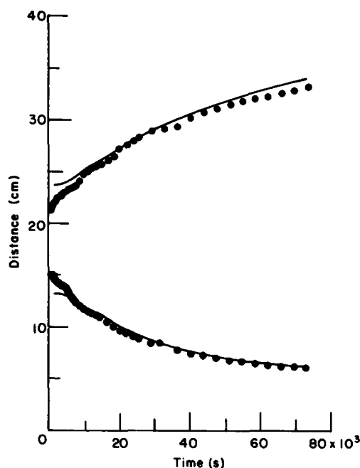
Figure 33. Phase front locations along the horizontal axis of symmetry for case 1. The solid line represents the numerical result, and the dots are locations interpolated from the data.
