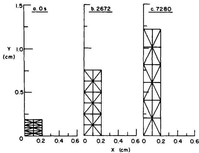
Figure 15. Initial, intermediate and final meshes for the Neumann comparison.
