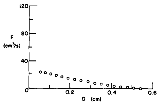
Figure 44. Flow rate F vs ice thickness D at the end of the 5-m pipe, in the case where the pipe freezes up.
