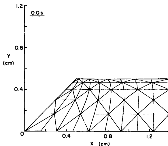
Figure 18. Initial mesh for the one-phase corner problem.
