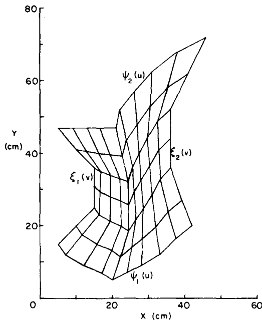
Figure 4. Use of the bilinear projector.
