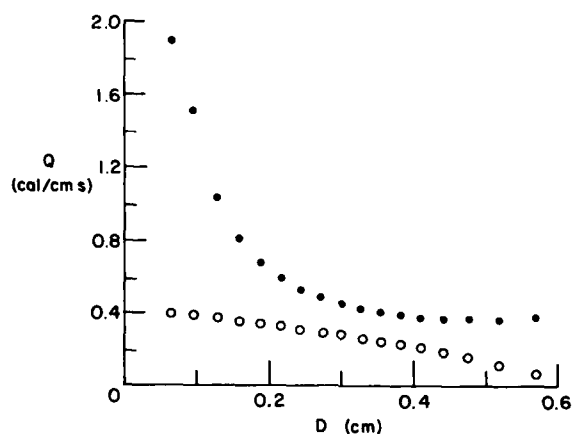
Figure 39. Heat flux Q vs ice thickness D at the end of the 1-m pipe, in the case where the pipe freezes up. The closed circles represent flux from the ice; the open circles represent flux from the water.
