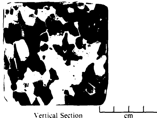
d. Columnar freshwater ice (Type IIC).
