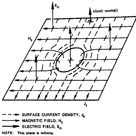
FIGURE A-4 FIELD VECTORS AND SURFACE CURRENT AT APERTURE
