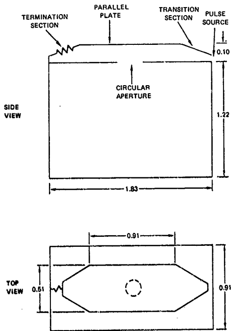
FIGURE A-3: TEST CONFIGURATION (all dimensions in meters)
