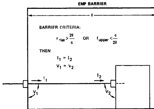
FIGURE 17 LIMIT ON RATE OF RISE OR BANDWIDTH INSIDE EMP BARRIER
