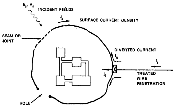
FIGURE 7 SHIELDED VOLUME WITH APERTURES AND WIRE PENETRATIONS
