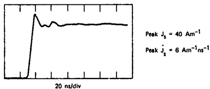
(a) SURFACE CURRENT DENSITY AT APERTURE
