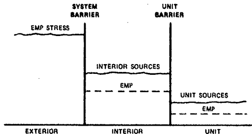
FIGURE 16 "FIRST BARRIER" ALLOCATION (only system barrier has EMP-unique requirement)
