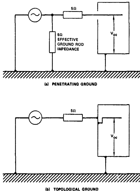
FIGURE 3 TEST SETUP (symbolic)
