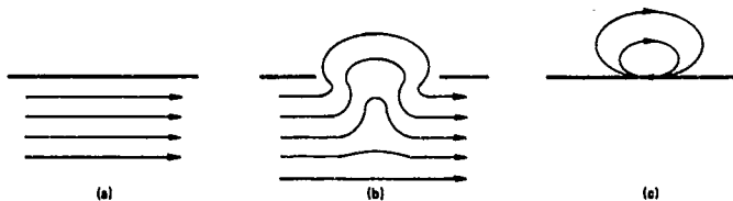
FIGURE 10 MAGNETIC FIELD APERTURE-COUPPING GEOMETRY. (a) Impressed magnetic field parallel to screen with no aperture. (b) Magnetic field near aperture in screen. (c) Equivalent magnetic dipole (on screen with no aperture) and its magnetic field far from aperture.
