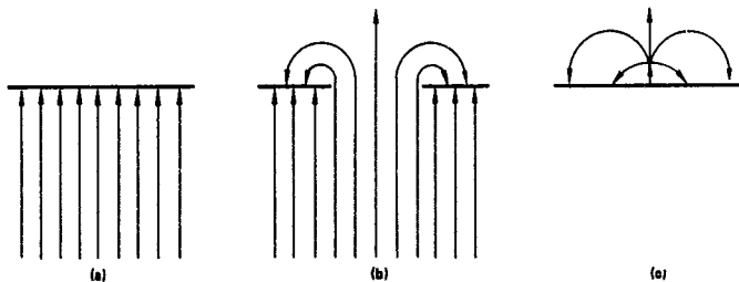
FIGURE 9 ELECTRIC FIELD APERTURE-COUPPING GEOMETRY. (a) Impressed electric field perpendicular to screen with no aperture. (b) Electric field near aperture in screen. (c) Equivalent electric dipole (on screen with no aperture) and its electric field far from aperture.
