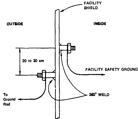
FIGURE 1 INTERNAL AND EXTERNAL GROUND CONNECTIONS
