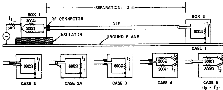
(a) TEST SETUP; ONLY TERMINATIONS AT BOX 2 WERE VARIED
