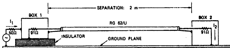
(a) TEST SETUP; CASE 2
