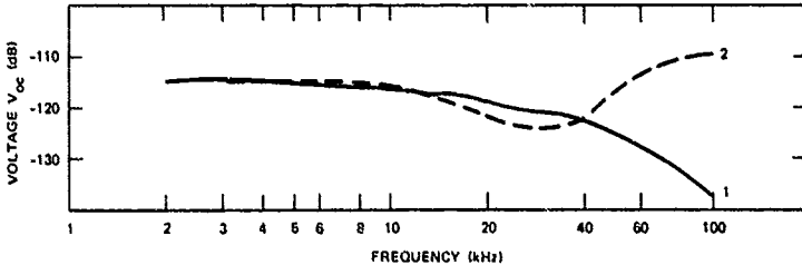
FIGURE 4 OPEN-CIRCUIT VOLTAGE V_{oc} AS A FUNCTION OF FREQUENCY. Setup as in Figure 3b. (1) box closed, (2) lid removed.
