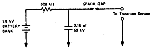
FIGURE A-6 PULSE SOURCE FOR PARALLEL PLATE REGION
