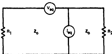
FIGURE A-2: GEOMETRY OF WIRE BEHIND APERTURE AND TRANSMISSION LINE COUPLING MODEL
