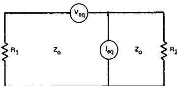
FIGURE 13 GEOMETRY OF WIRE BEHIND APERTURE AND TRANSMISSION LINE COUPLING MODEL
