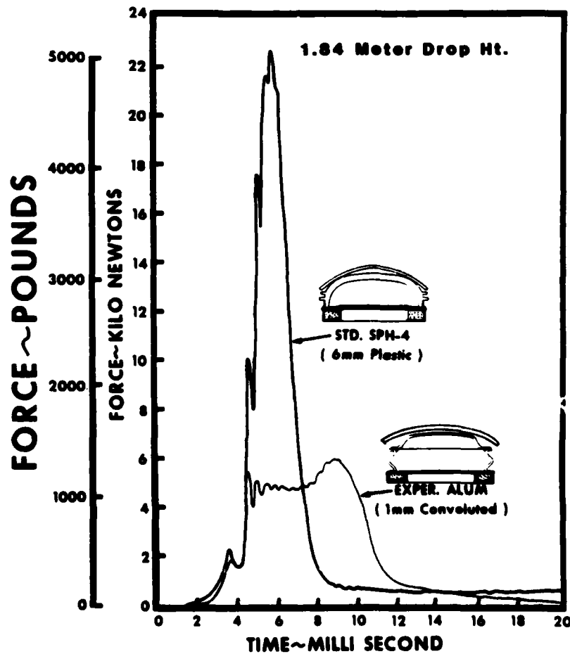
FIGURE 17. Comparison of the Dynamic Loading Performance of the Convoluted Aluminum Earcup and the Standard SPH-4 Earcup
