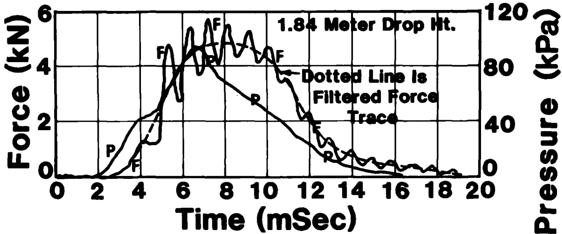
FIGURE 11. Dynamic Crushing Load and Pressure Rise of Foam Energy-Absorbing Earcup
