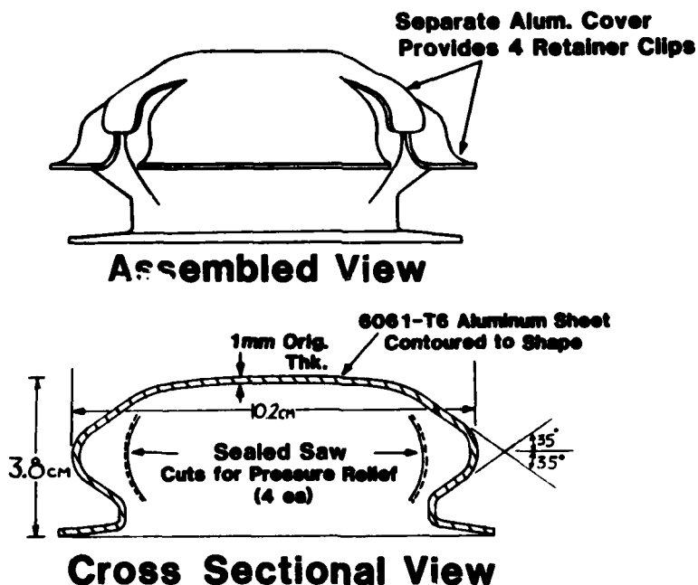
FIGURE 7. Crushable Aluminum Earmuff as Redesigned by Simula, Inc.
