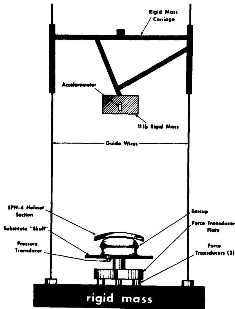
Earcup Test Set-up
