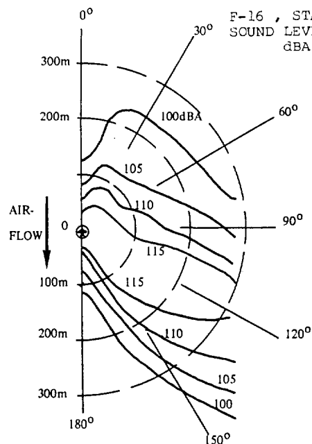
Fig 21: MAX AFTERBURNING
