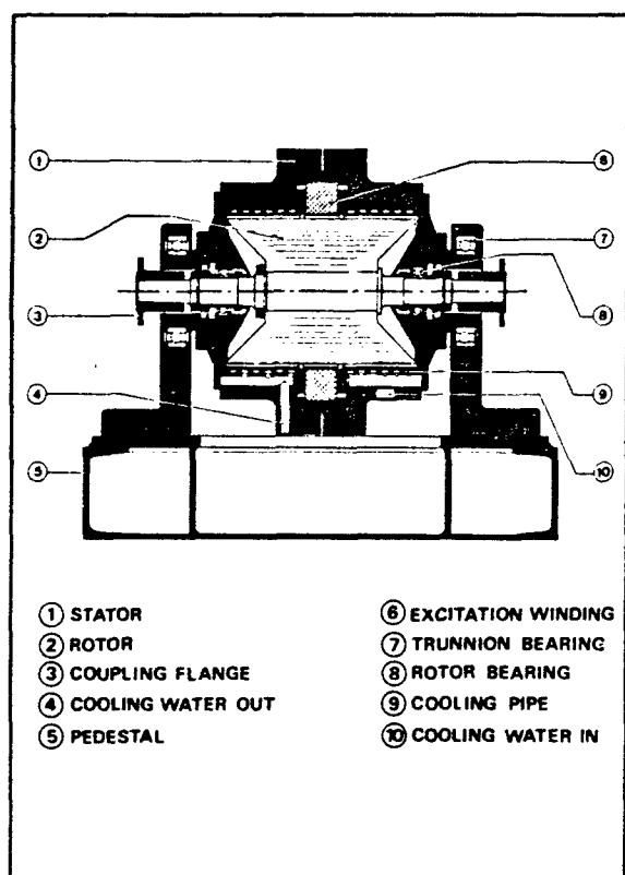
Fig. 4 Eddy-current dynamometer
