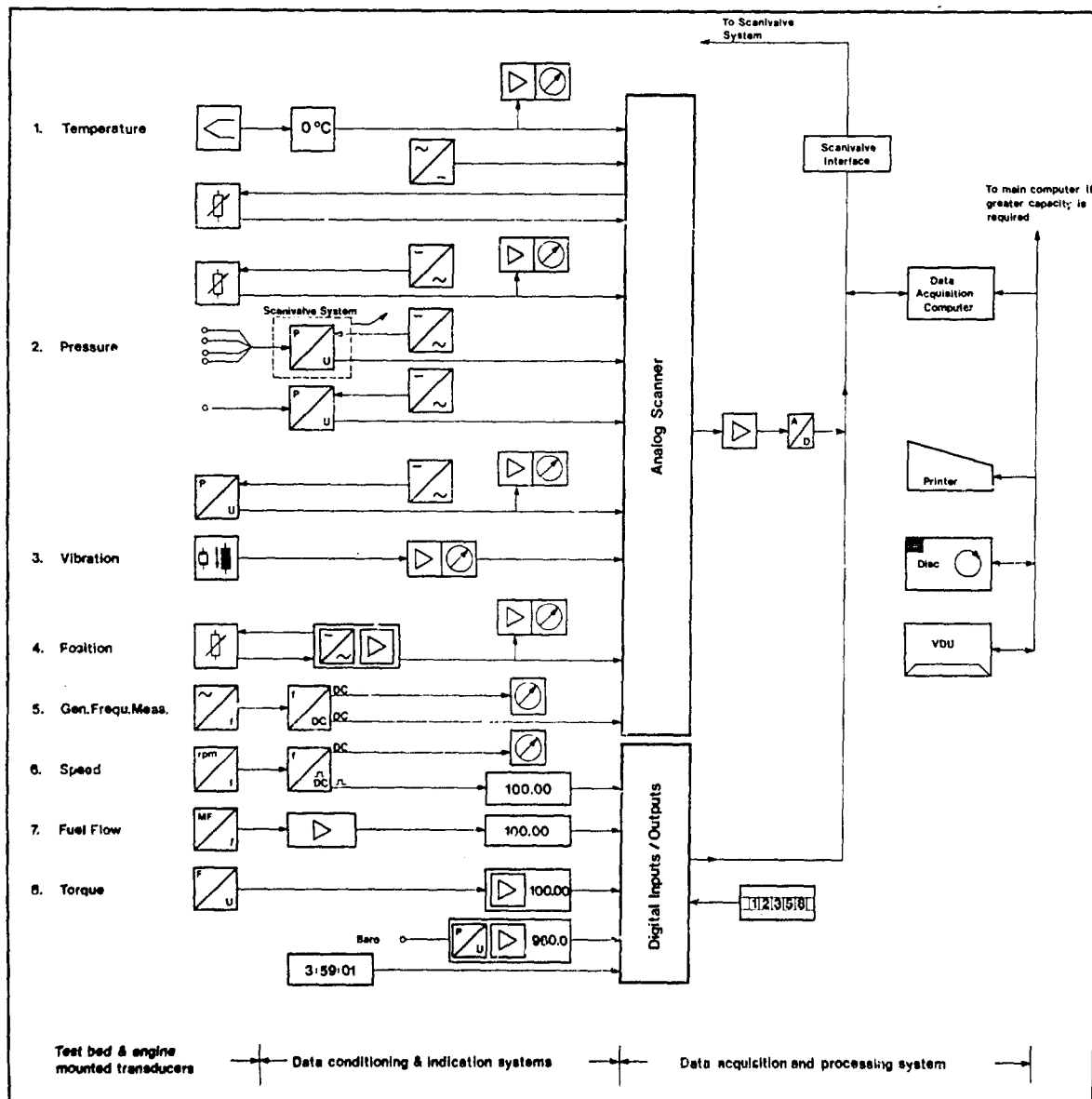
Fig. 7 Static measuring equipment for engine test facility
