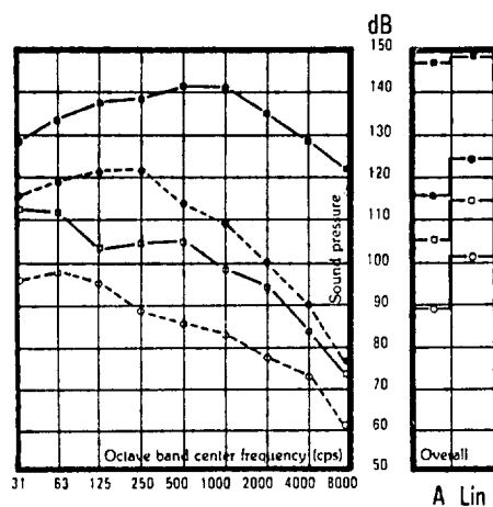
Fig 23: IDLE
