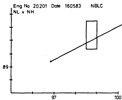
Figure 8 Spey 202 HP9826 Display (1)
