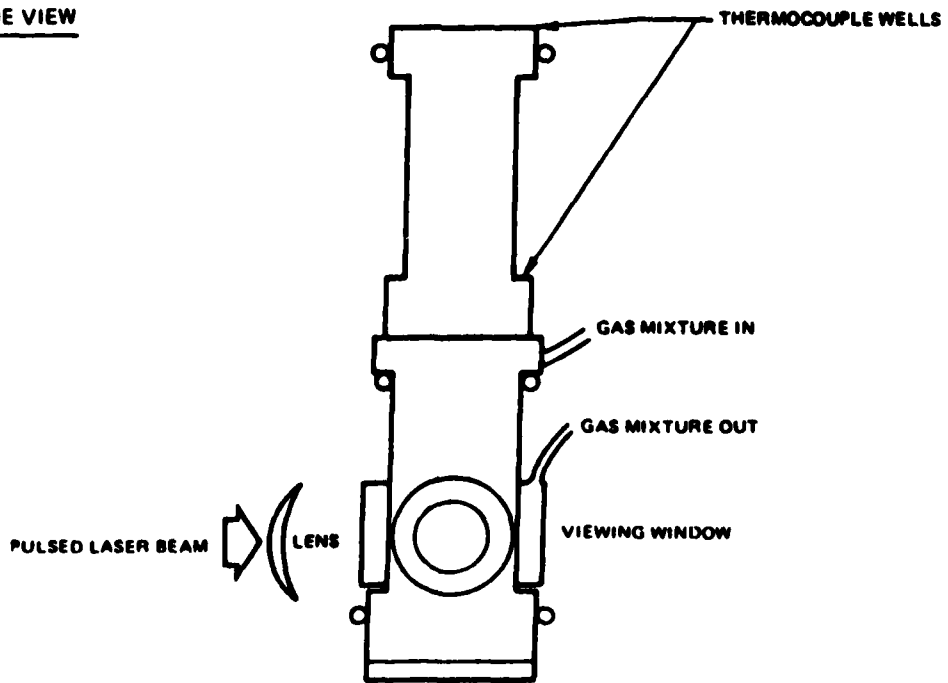
Figure A-6. The UTRC High Pressure Gas Cell.
