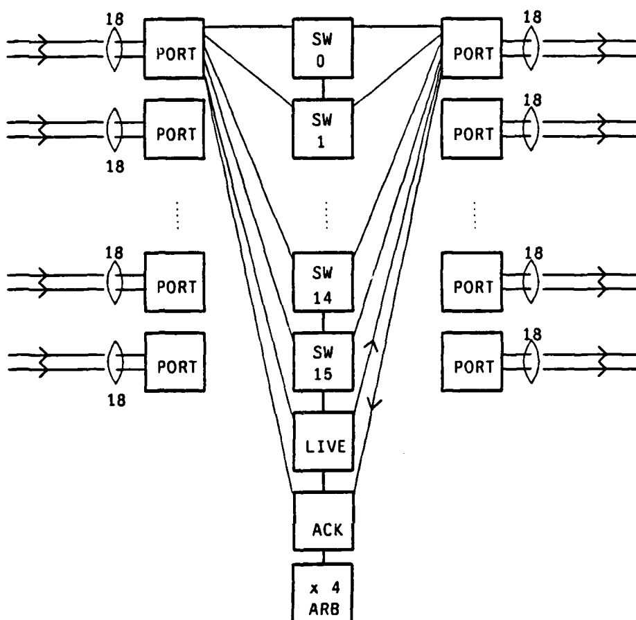
Figure 14: Eighteen bit slice crosspoint chips interconnect a society of RAPIDbus II processor nodes.
