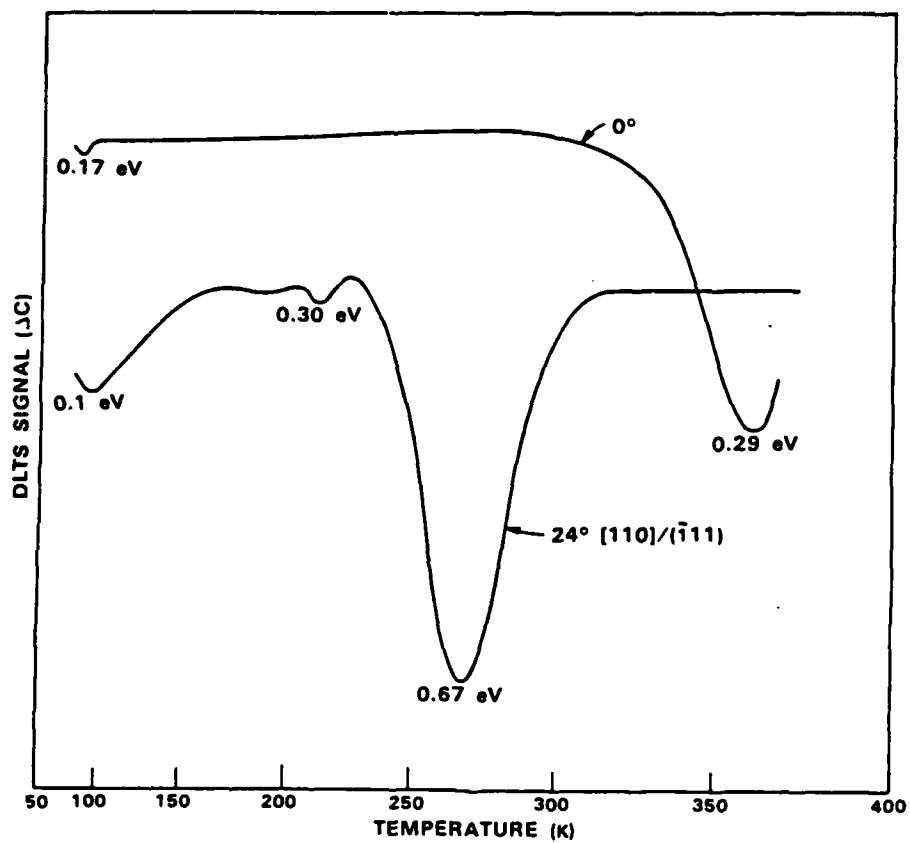
Fig. 7-7. DLTS spectra for 0 and 24° bicrystal layers. Activation energies of the traps are indicated.
