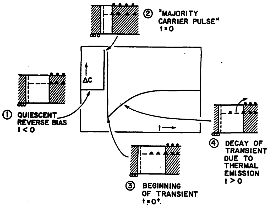
Fig. 9-2. Schematic illustration of capacitance transient for isothermal emission from a majority carrier trap. Inserts show the p^+n junction configuration at various times during the transient [Lang (121)].
