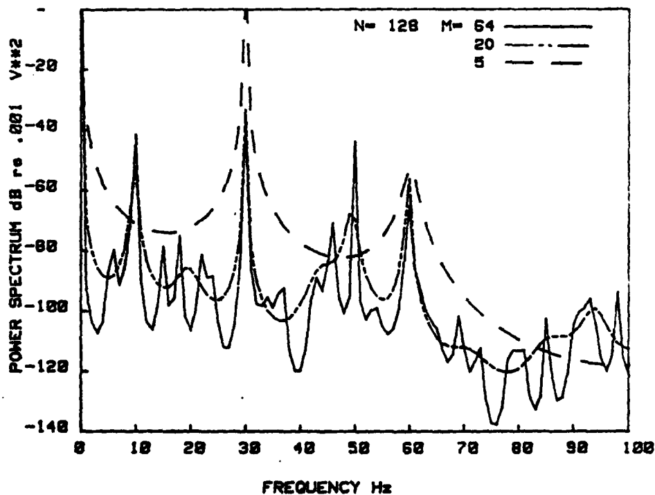
FIGURE 14. MESA PERFORMANCE ON MACHINERY NOISE Sampling Frequency 200Hz
