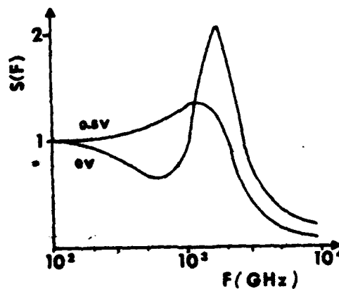
Noise spectral density
