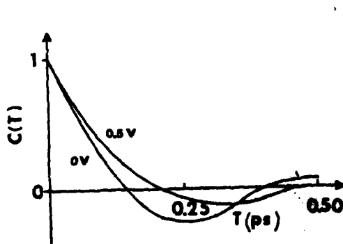
Correlation function of current noise
