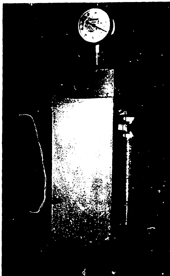
Figure 4. Comparator used for checking the flatness and parallelism of specimen end planes (a) and the parallelism of bonded end caps (b).
