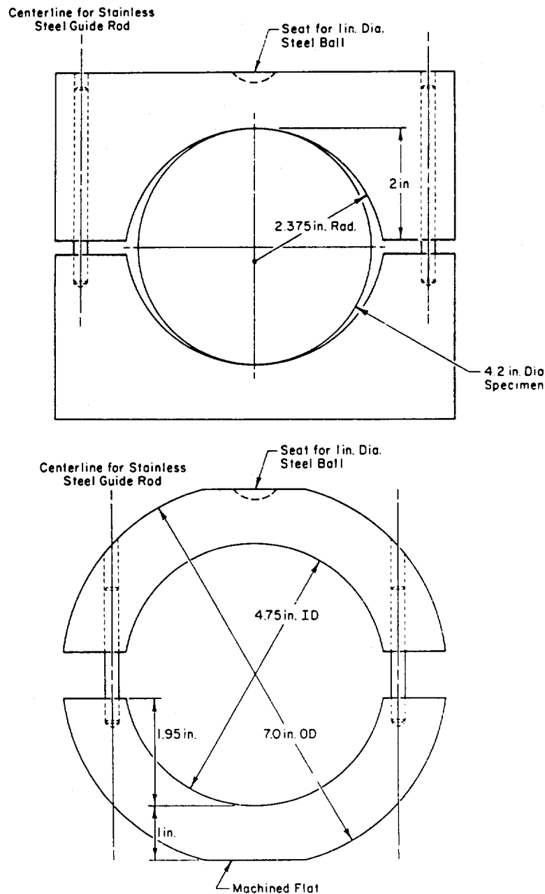
Figure E1. Loading frame for making diametral compression tests.
