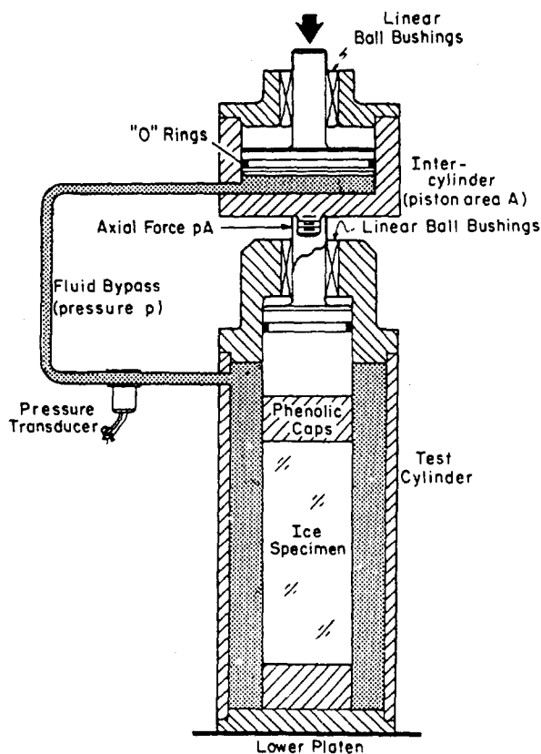
Figure 18. Diagram of the triaxial compression test equipment.
