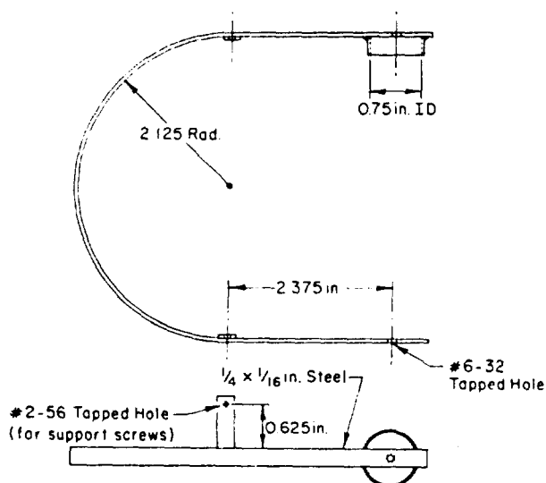
Figure 25. Details of original (MkII) yoke for measuring radial strains.
