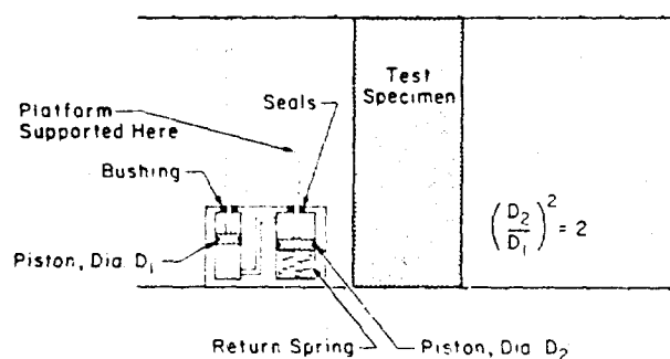
Figure 26. Hydraulic device for supporting an instrument platform at the level of the specimen mid-plane.
