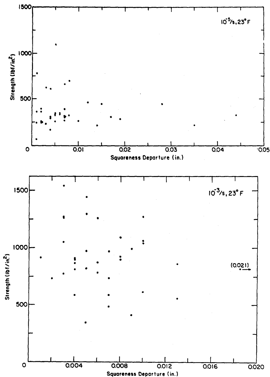
Figure 12. Measured uniaxial compressive strength plotted against squareness departure for tests at -5^{\circ}C ( 23^{\circ}F ), with strain rates of 10^{-5}/s and 10^{-3}/s .
