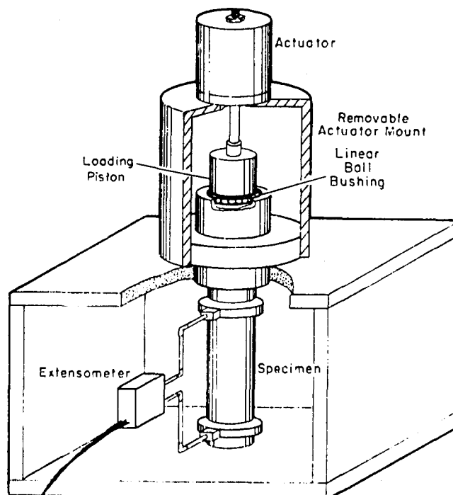
b. Modified apparatus of Mellor and Cole.
