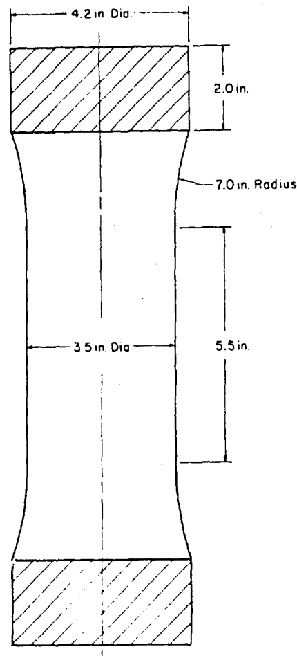
Figure 10. Geometry of tensile specimen.
