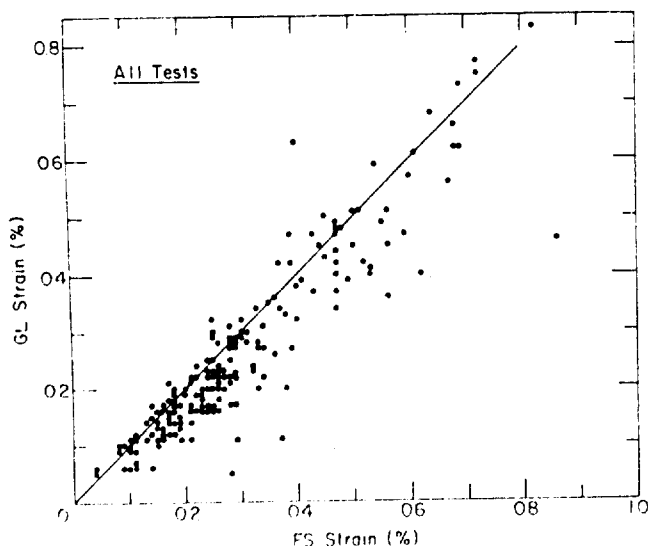
Figure 24. Comparison between full-sample and gauge-length strain measurements.
