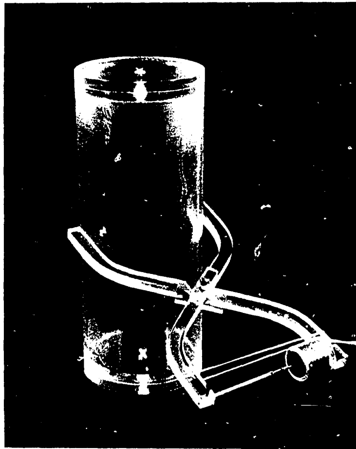
Figure D4. Scissors-type caliper for measuring radial strains.
