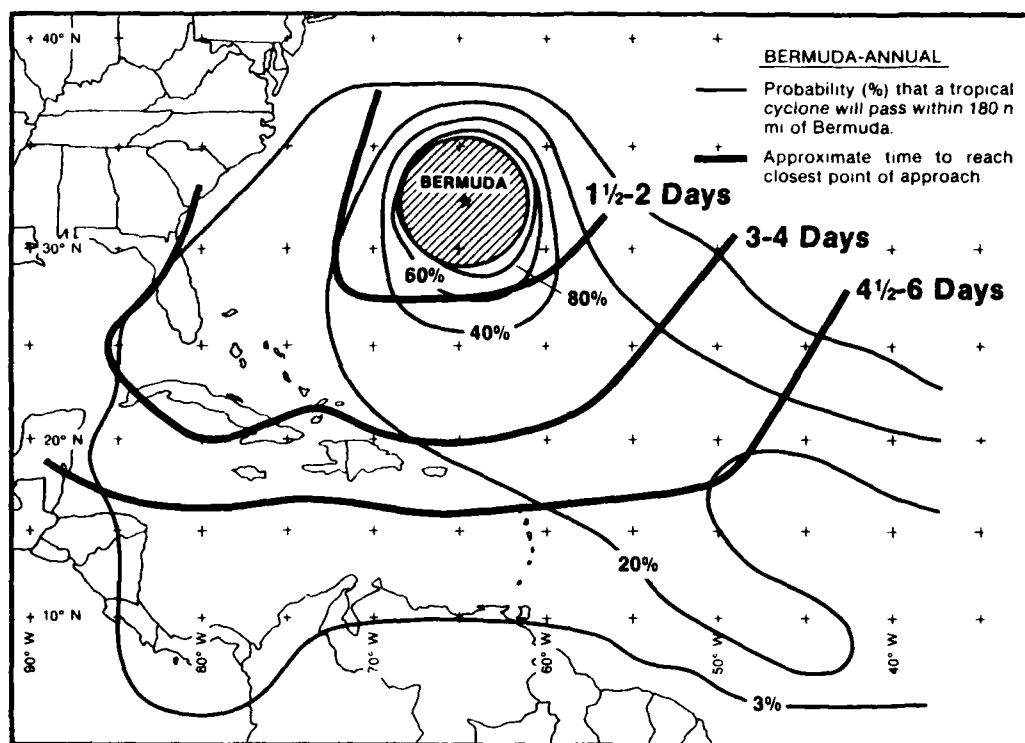
Figure XXII-14. Annual probability and CPA curves for all tropical cyclones passing within 180 n mi of Bermuda during the years 1871-1979.
