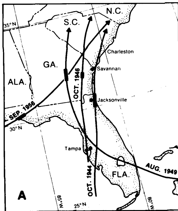
Figure XVIII-9. Eight tropical cyclones have produced sustained winds of gale force in Savannah since 1940. Four of these events have occurred with decaying storm systems which had tracked overland (A). The strongest winds and highest tides in Savannah have been associated with those tropical cyclones which have moved from the east or east-southeast, as the October 1947 hurricane (B). The heavy lines superimposed on the storm tracks represent the center position during the time period that wind conditions of gale force or higher were recorded in Savannah. At other times sustained wind speeds in Savannah were below 34 kt.
