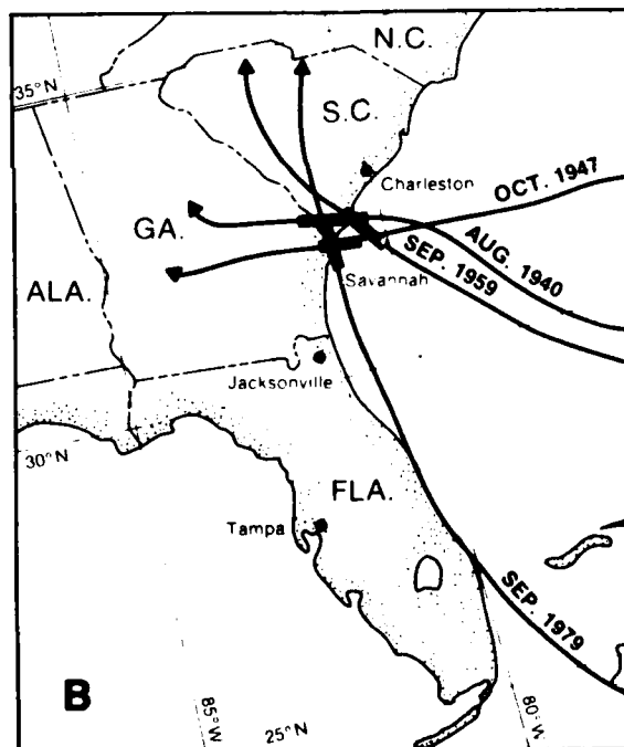
Figure XVIII-9. Eight tropical cyclones have produced sustained winds of gale force in Savannah since 1940. Four of these events have occurred with decaying storm systems which had tracked overland (A). The strongest winds and highest tides in Savannah have been associated with those tropical cyclones which have moved from the east or east-southeast, as the October 1947 hurricane (B). The heavy lines superimposed on the storm tracks represent the center position during the time period that wind conditions of gale force or higher were recorded in Savannah. At other times sustained wind speeds in Savannah were below 34 kt.
