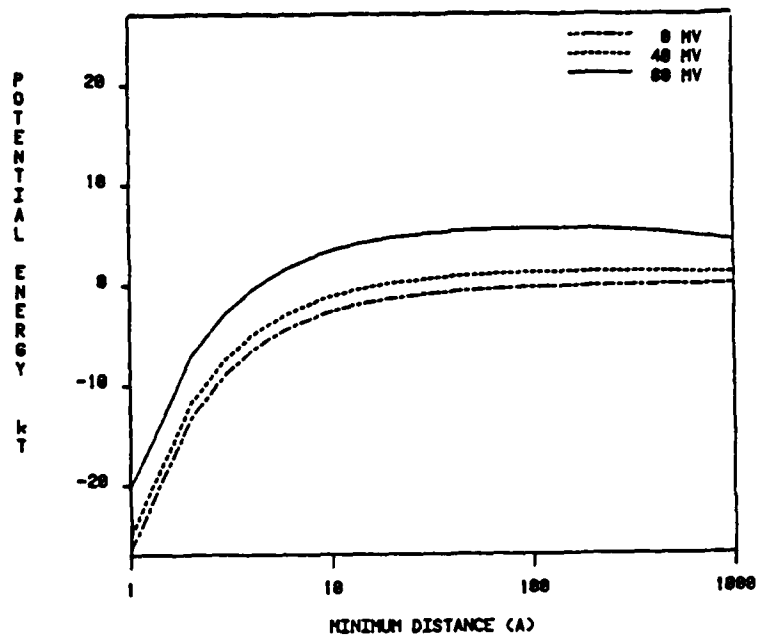
Figure V.4. Interparticle energies for silicon in n-propanol as functions of interparticle distance and surface charge. Radius = 400\text{\AA} ; [\text{ion}] = 1 \times 10^{-9} \text{ m} ; T = 300^\circ\text{K} .
