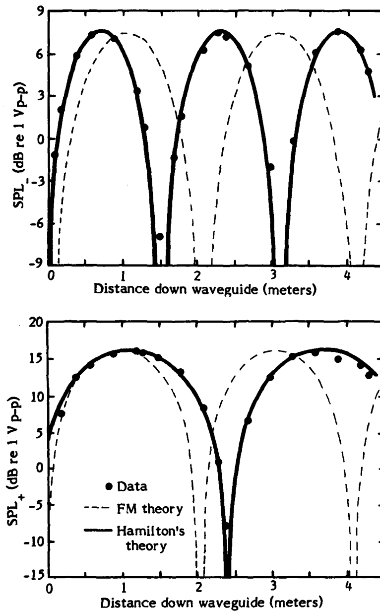
Figure 4.7 Comparison of observed data with predicted periodicity of the sum and difference frequency wave amplitudes
