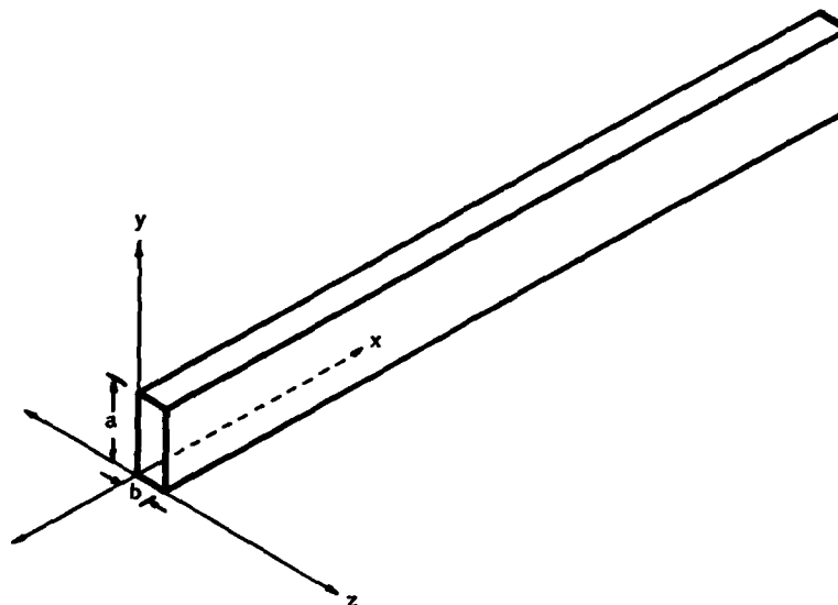
Figure 2.4 Waveguide geometry
