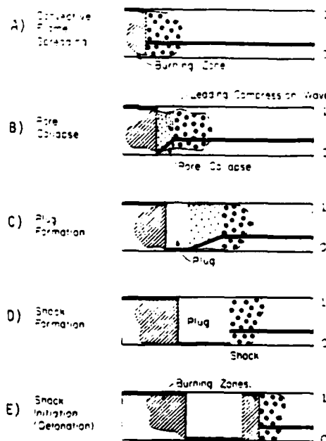
Fig. 5. Five-part sequence of events leading to DSDT.
