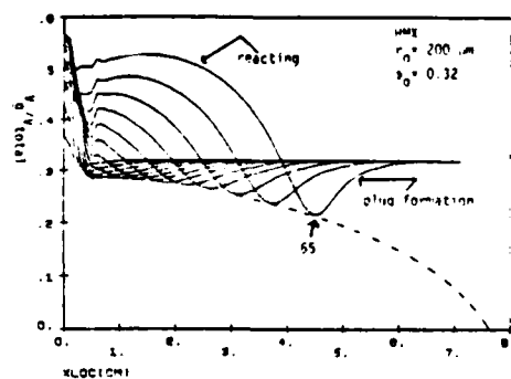
Fig. 8 Volume fraction of gas phase showing complete plug formation ( \delta=0 ) for HMX, 200 \mu\text{m} .
