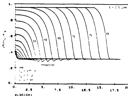
Fig. 5 Volume fraction of gas phase showing compaction in early times (50 to 65 μsec).
