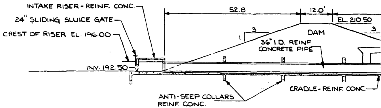
PROFILE ALONG \phi OF PRINCIP
