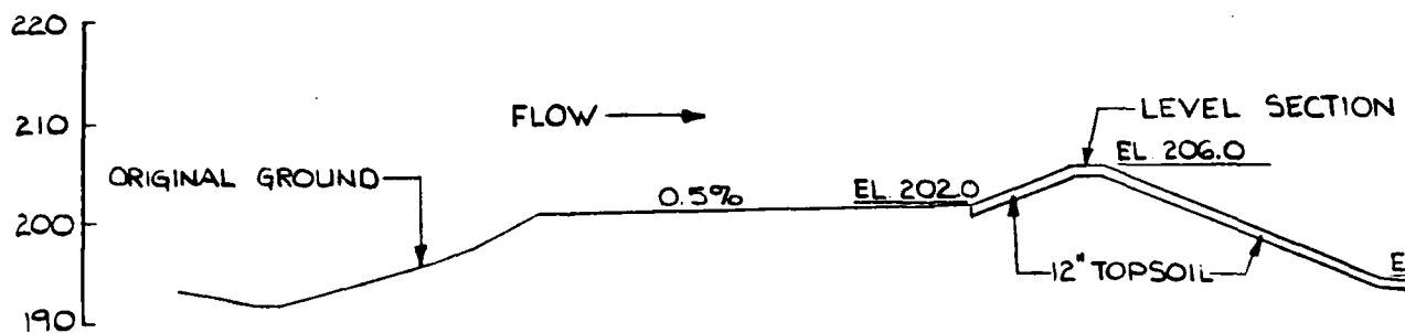
PROFILE ALONG \phi OF EMERGENCY SPILLWAY
