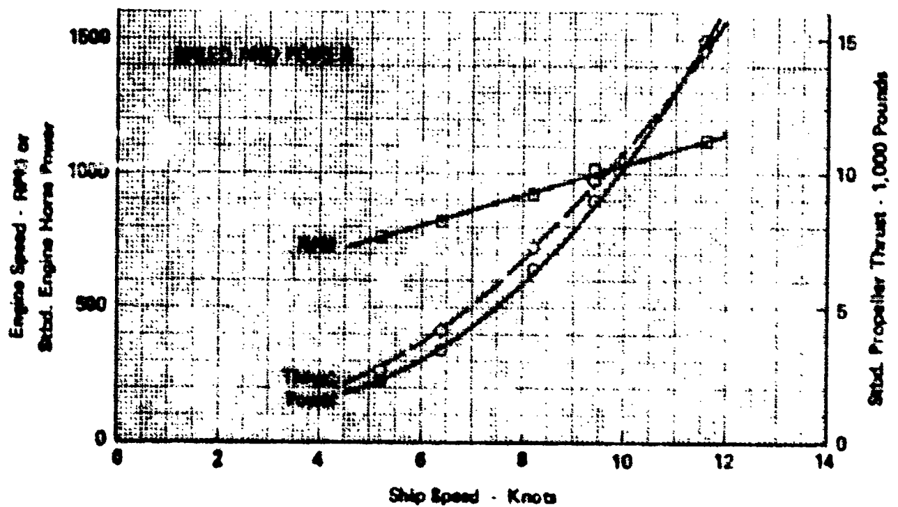
Figure 13 - Single Engine Hullborne Performance
