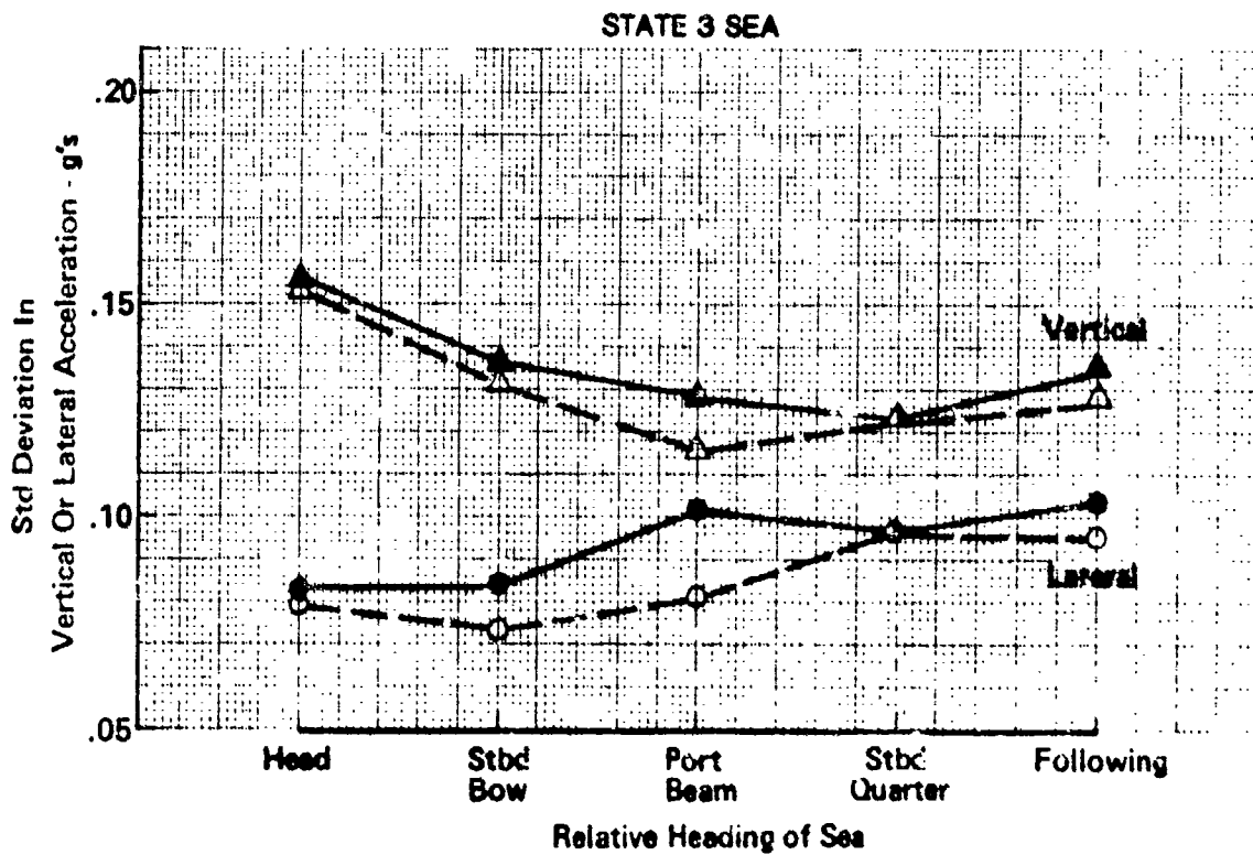
Figure 56 - Pilot House Lateral and Vertical Accelerations
