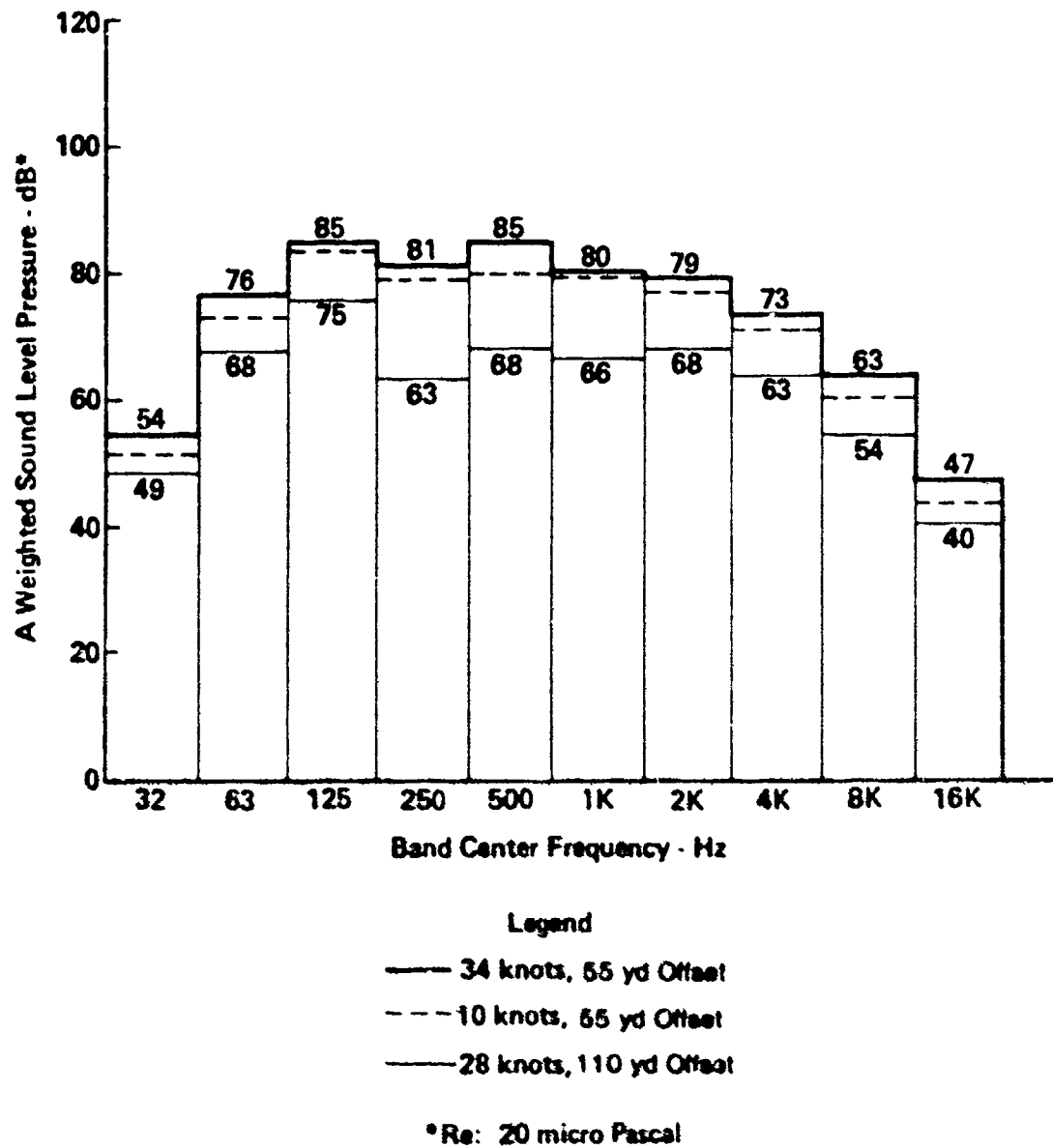
Figure 36 - Broadside Transmitted Sound Levels
