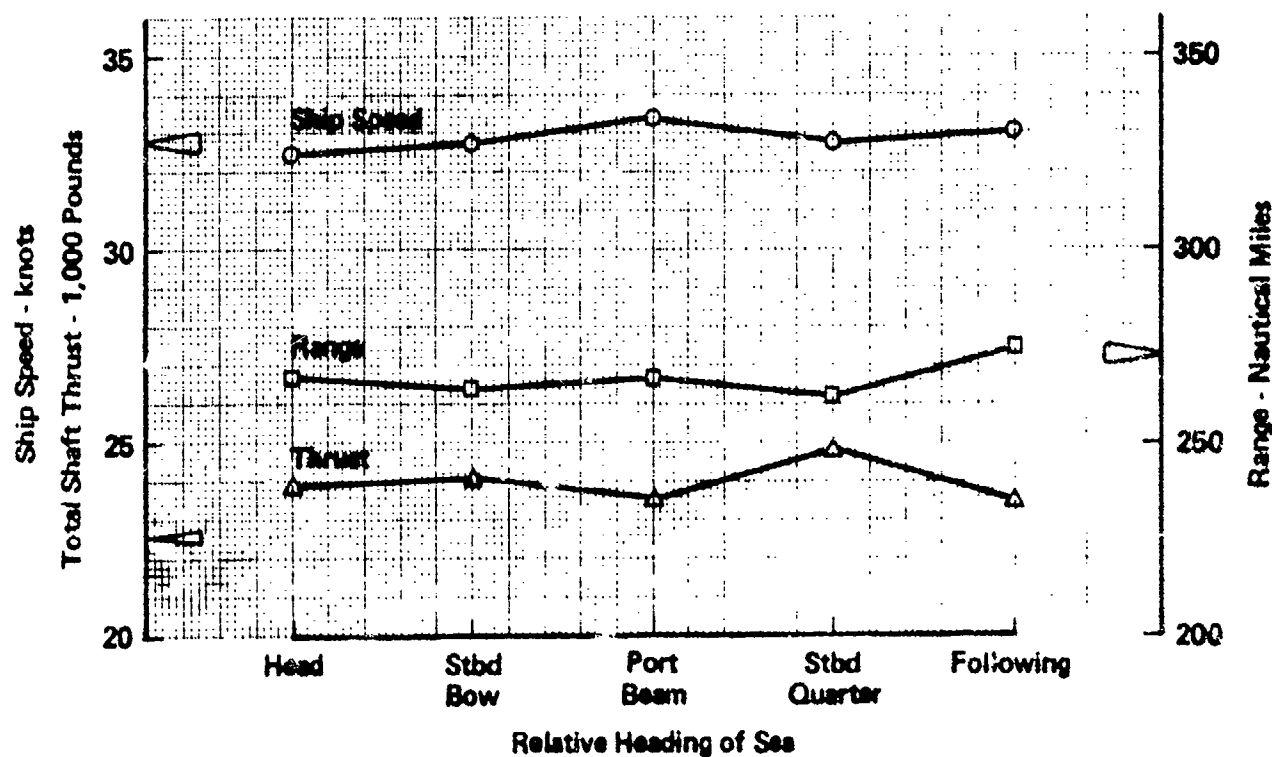
Figure 48 - Foilborne Speed and Power in State 3 Seas - SAS Active
