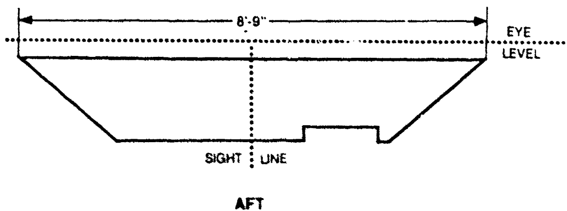
Figure 75. Pilot House Visibility From Captain's Chair
