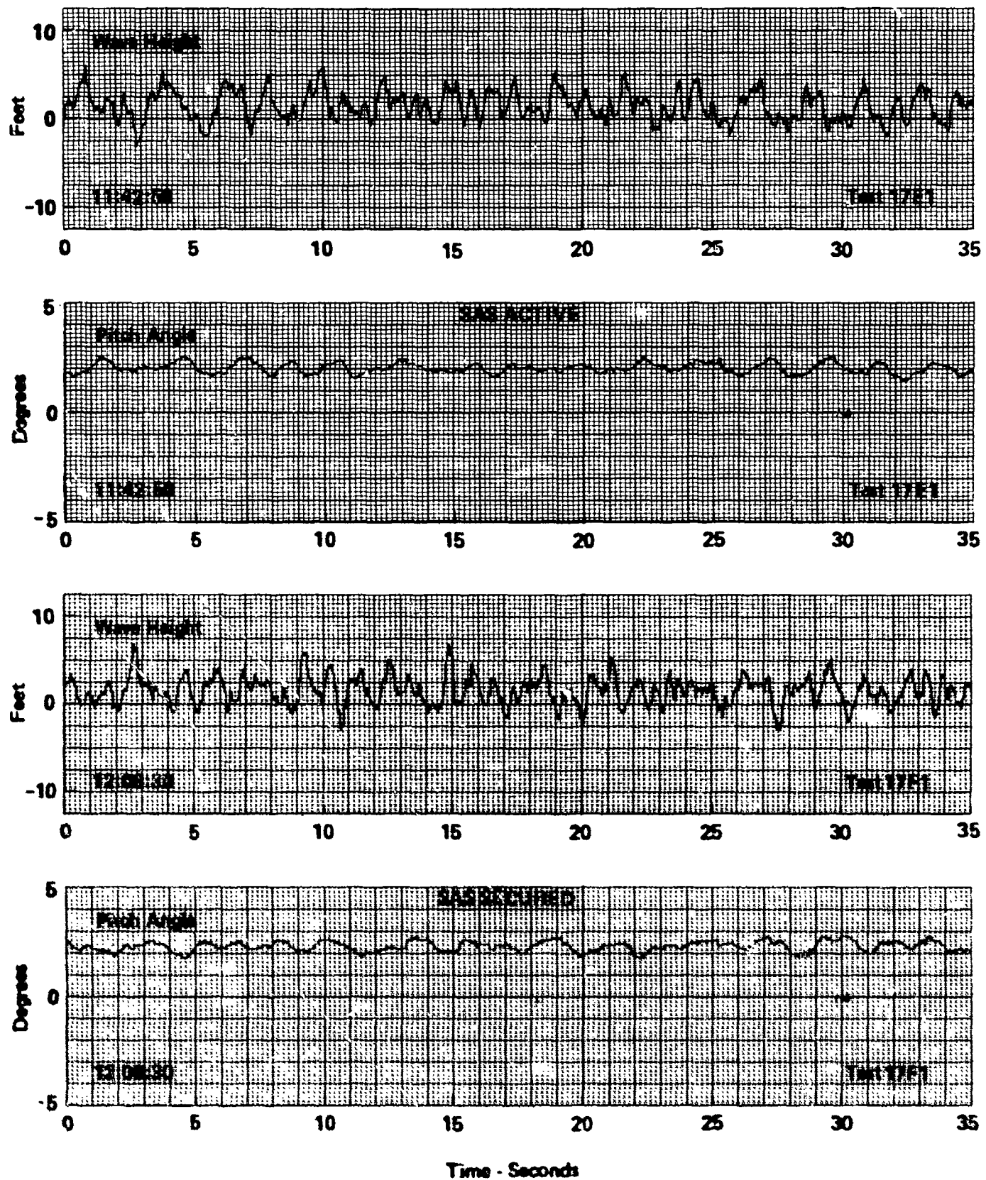
Figure 58 - Pitch Response in State 3 Head Seas
