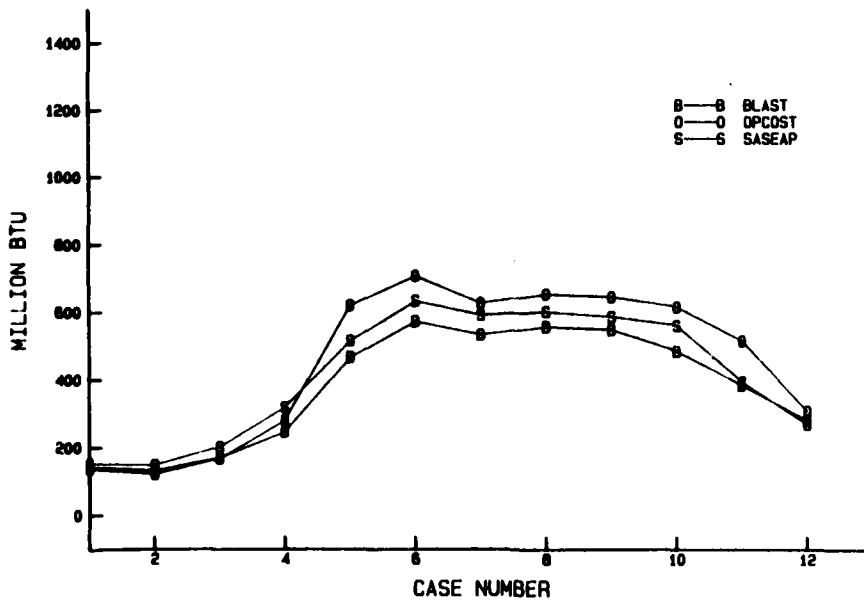
Figure 8. Total energy consumption at the three locations.
