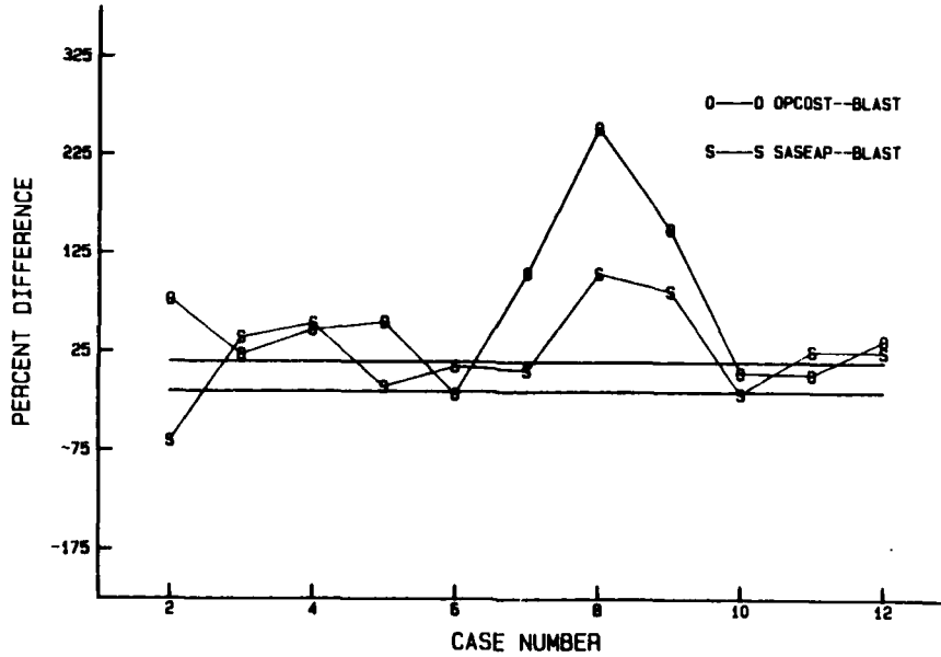
Figure 11. Deviations between BLAST-computed and micro-computed energy savings.
