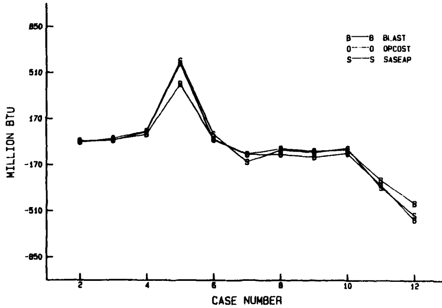
Figure 10. Impact of design features on energy consumption.
