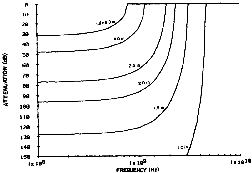
Figure 10. Theoretical attenuation of a 6-in. (15.25-cm) pipe filled with carbon tetrachloride ( \epsilon_r \approx 2 ) for various inside diameters.
