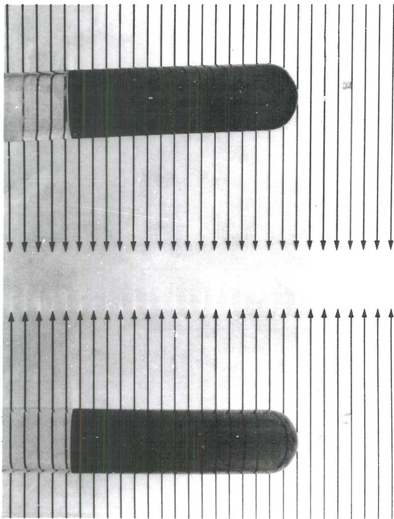
Figure 21. Sample of red fuel at the Cloud Point.
