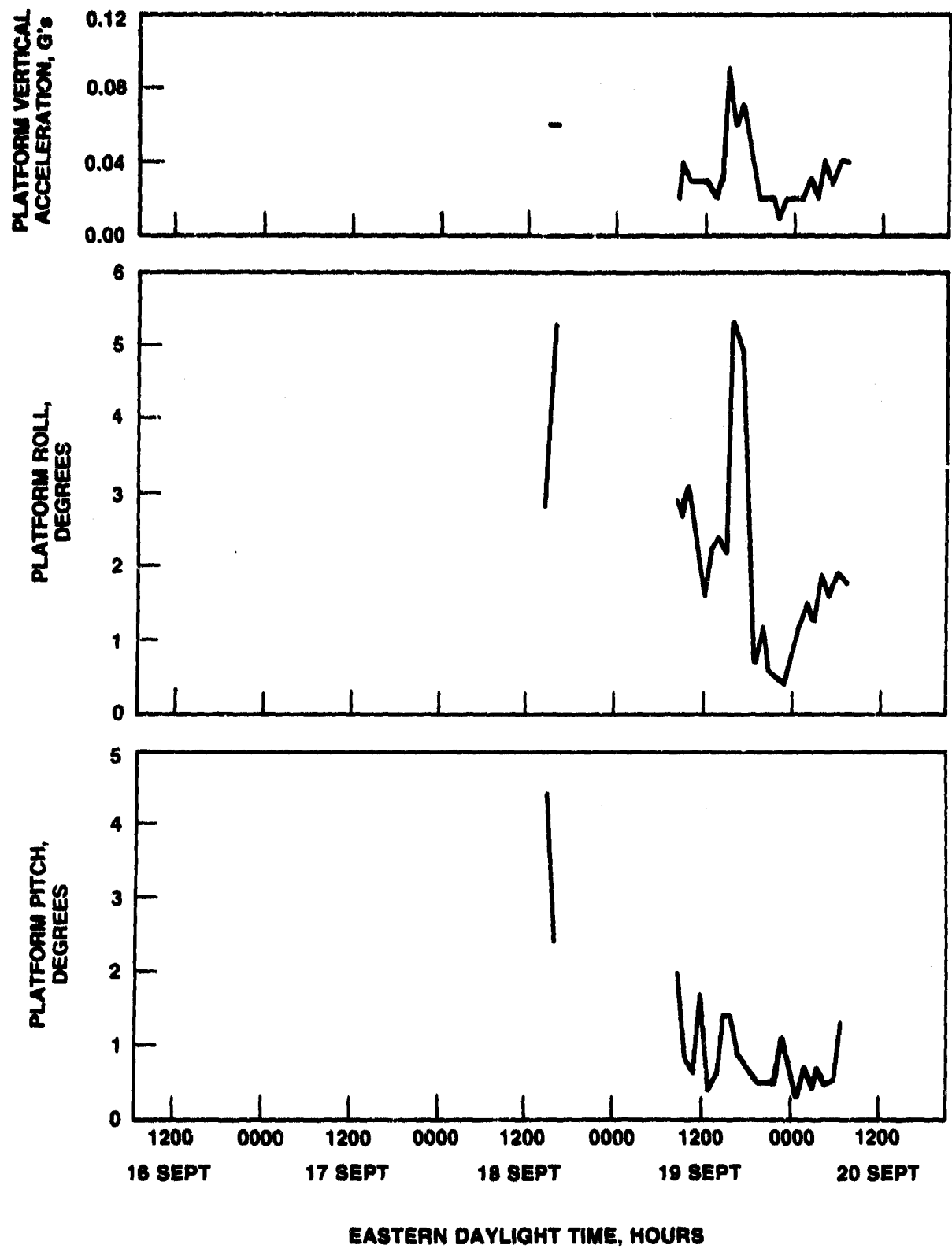
Figure 24 - Platform Motion Range Variations versus Date and Time Obtained during the Trial
