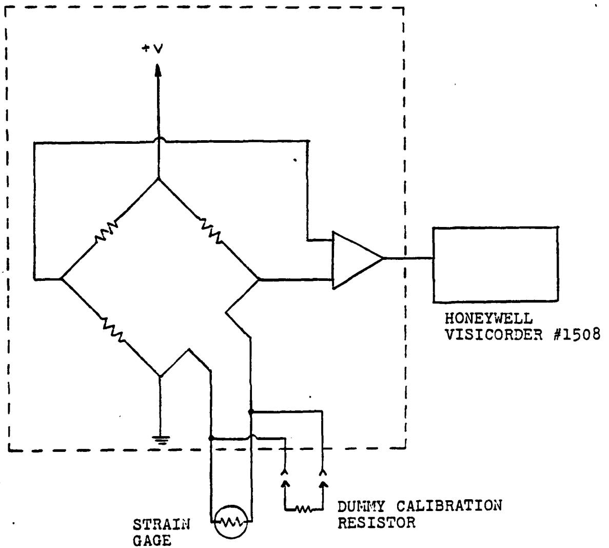
FIGURE 3.6: Strain Gage Instrumentation Circuit
