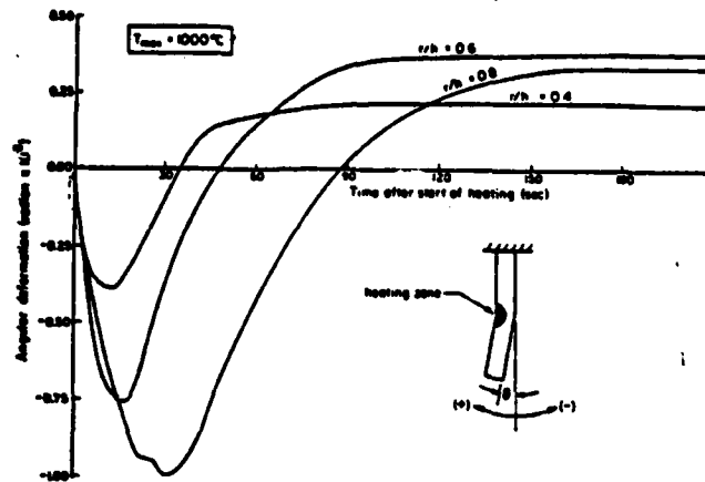
FIGURE 2.15: Transient angular deformation for various heated areas
