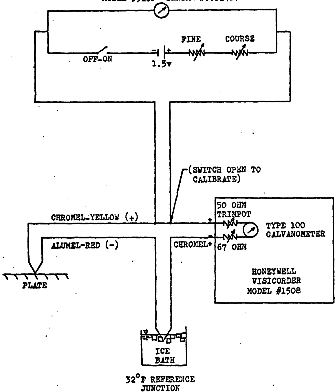
FIGURE 3.7: Thermocouple Instrumentation Circuit
