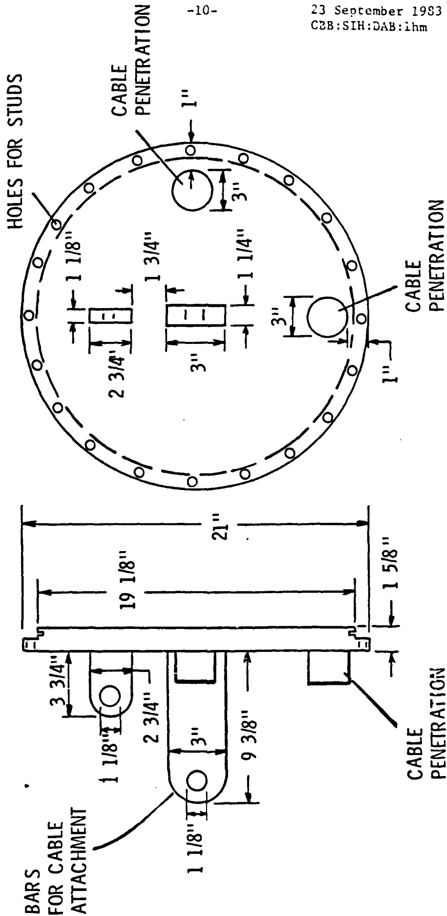
Figure 6. End Caps with Cable Penetrations
