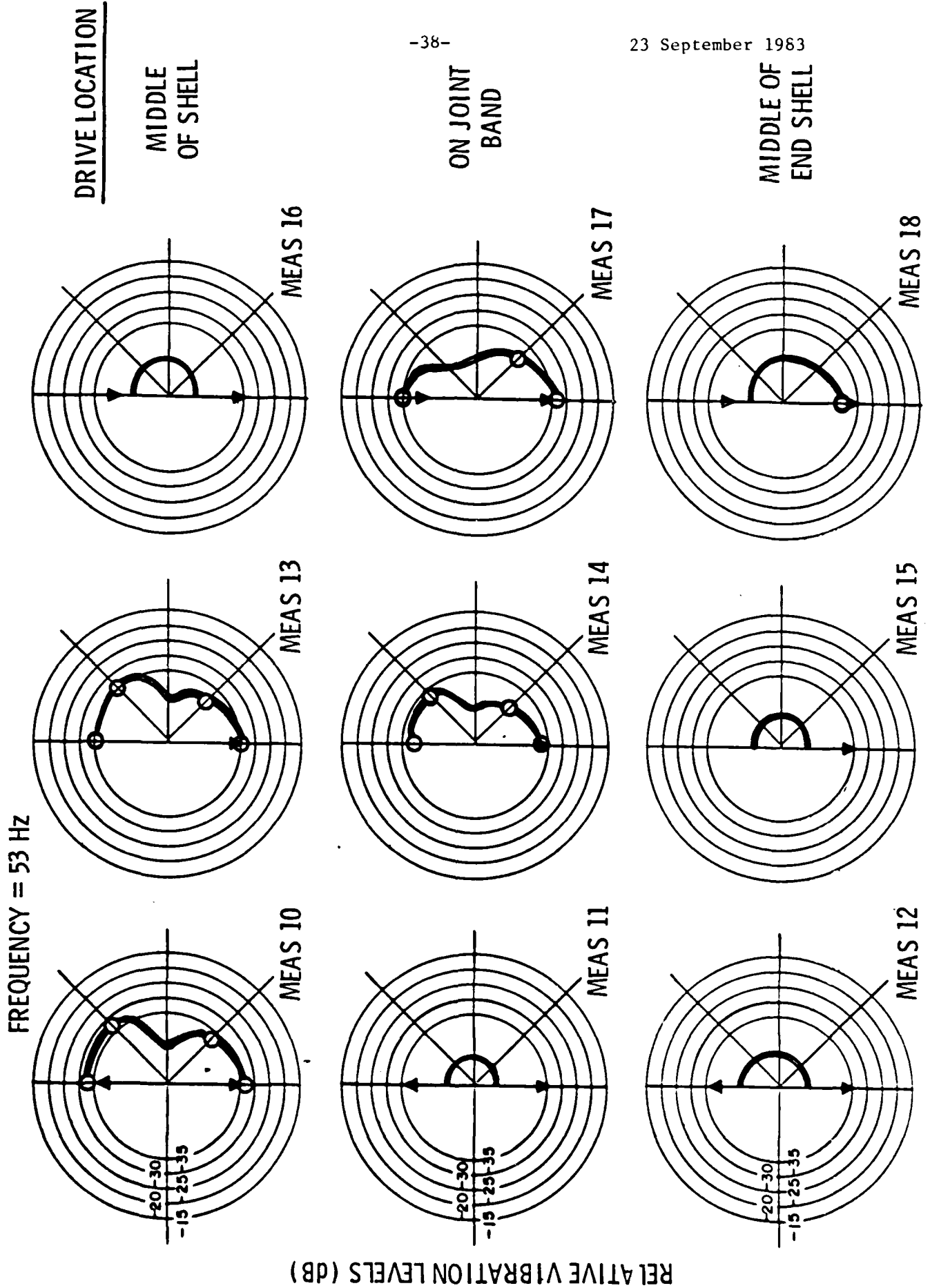
Fig. 18. Circumferential Mode Plots for Fig. 17, Cl. II in Air at 53 Hz
