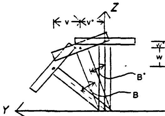
Figure (0-3) Tee Stiffener
