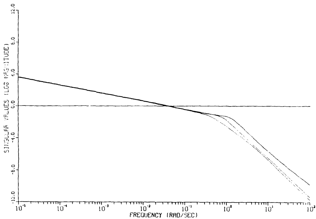
Figure 17. Singular values of \underline{T}(j.) .
