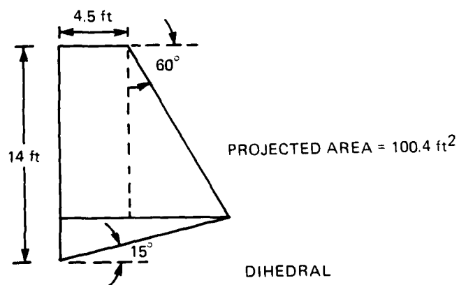
Figure 3. Rear view, rudder, and dihedral fin dimensions.
