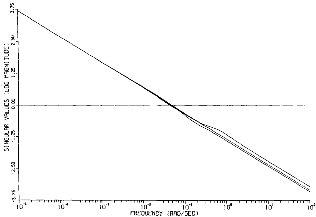
Figure 16. Singular values of \underline{G}_{KF}(j\omega) .
