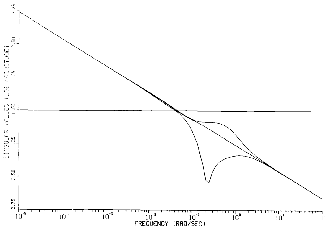
Figure 15. Singular values of \underline{G}_{FOL}(j\omega) .
