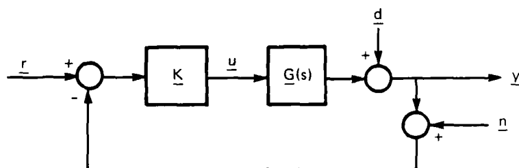
Figure 8. Generalized feedback loop.
