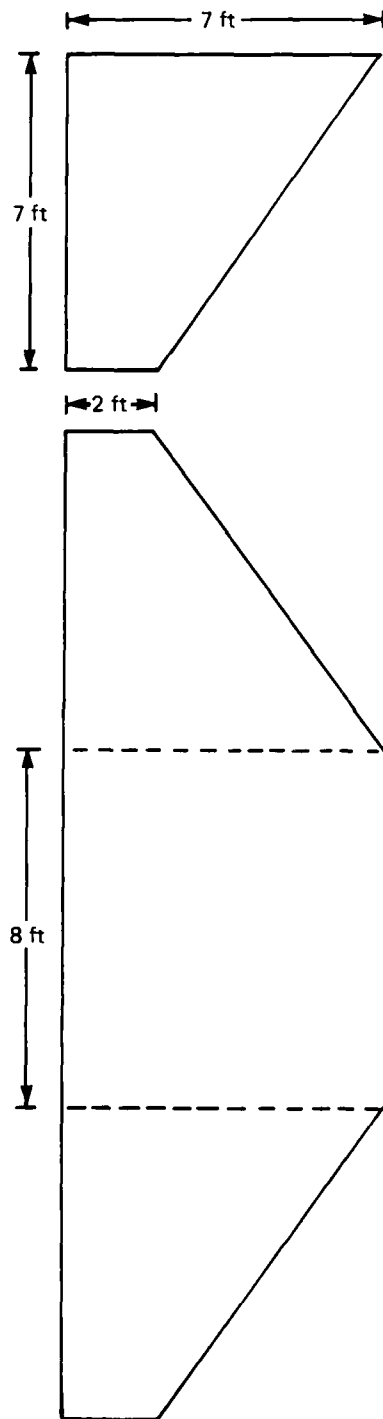
Figure 6. Sailplane geometry.
