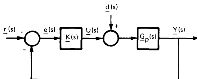
Figure 13. Feedback structure of a MIMO control system.
