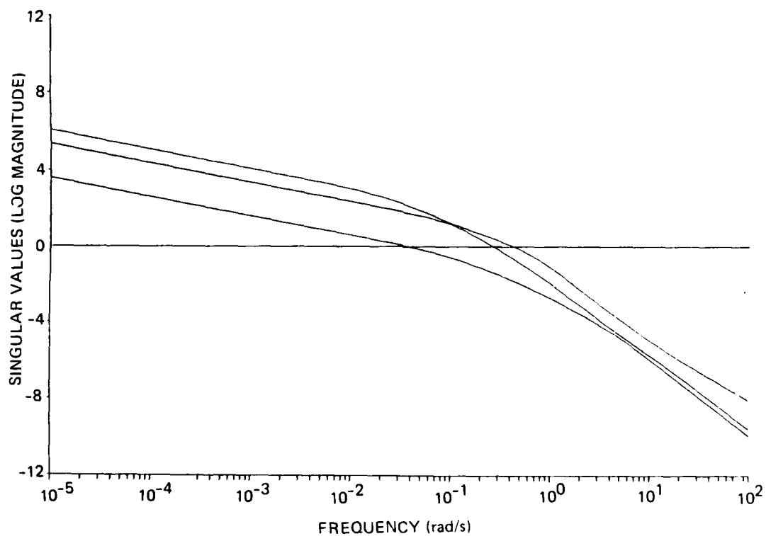
Figure 11. Singular values of open loop plant.
