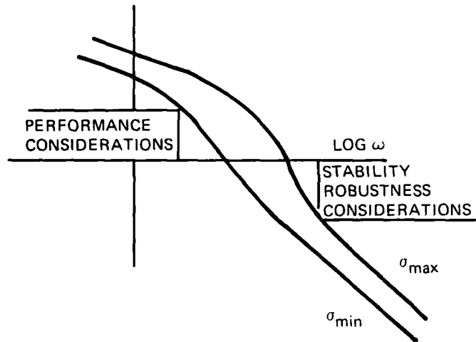
Figure 9. Frequency domain requirements.
