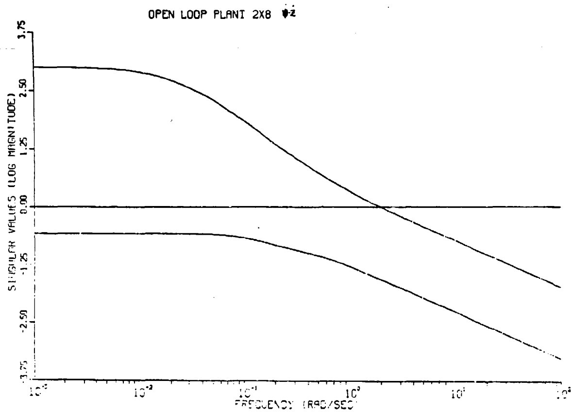
Figure 4-5. Unaugmented open-loop plant, \dot{\psi} - \dot{z} system; singular values vs frequency.
