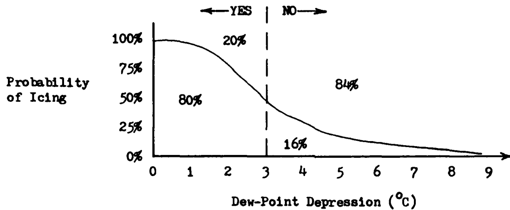
Figure 7.5 A graphical interpretation of the probability density curve for icing forecasts based on TR-80 paragraph 22.a and Table 2. Using a 3°C dew-point depression cut-off for forecasting icing, one would expect 20% of the YES forecasts to be false alarms and 80% to be hits. Similarly, 84% of the NO forecasts would be hits and 16% misses.
