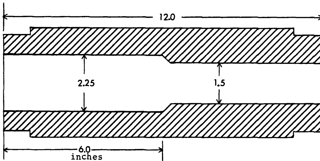
Figure 6. Partially Enlarged Fuel Grain.
