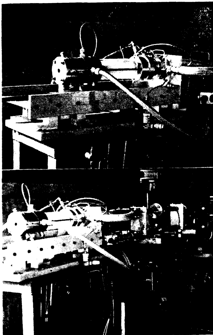
Figure 3. Photographs of Solid Fuel Ramjet Assembly
