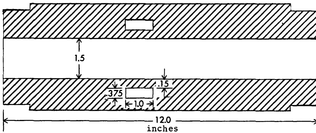
Figure 5. Fuel Grain with Slot.
