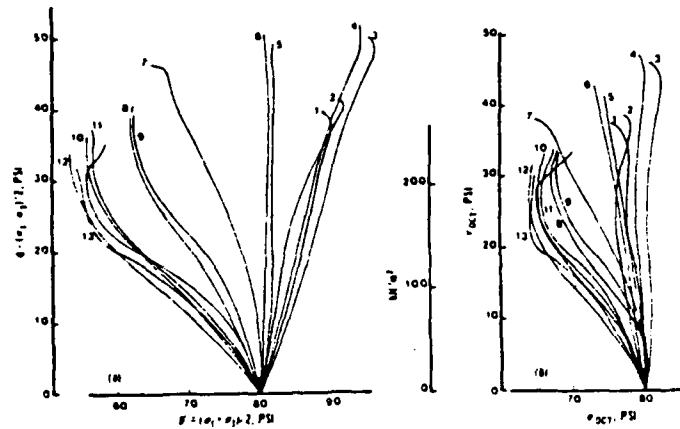
Figure 19. Effective Stress Paths for Florida-1 Clay (24)
