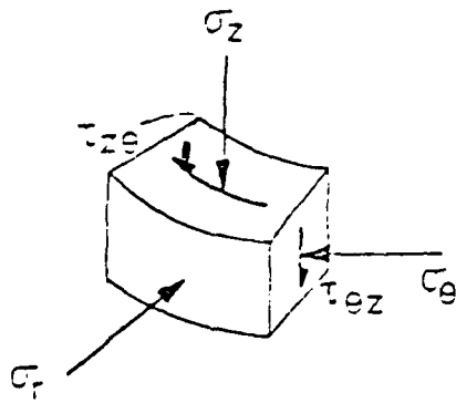
Figure 4. Stresses in the Hollow Cylinder Specimen
