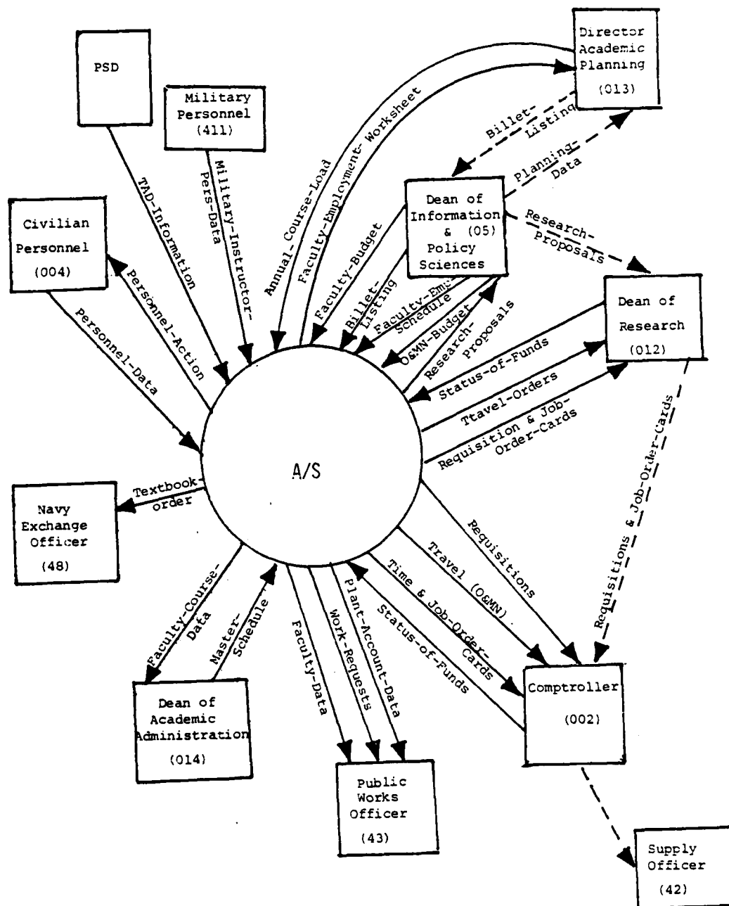
Figure 3-2 The Context Diagram
