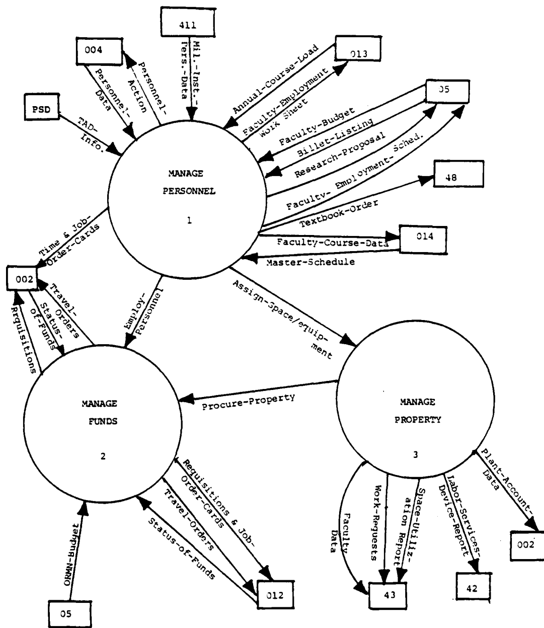
Figure 3-3 Level One Decomposition
