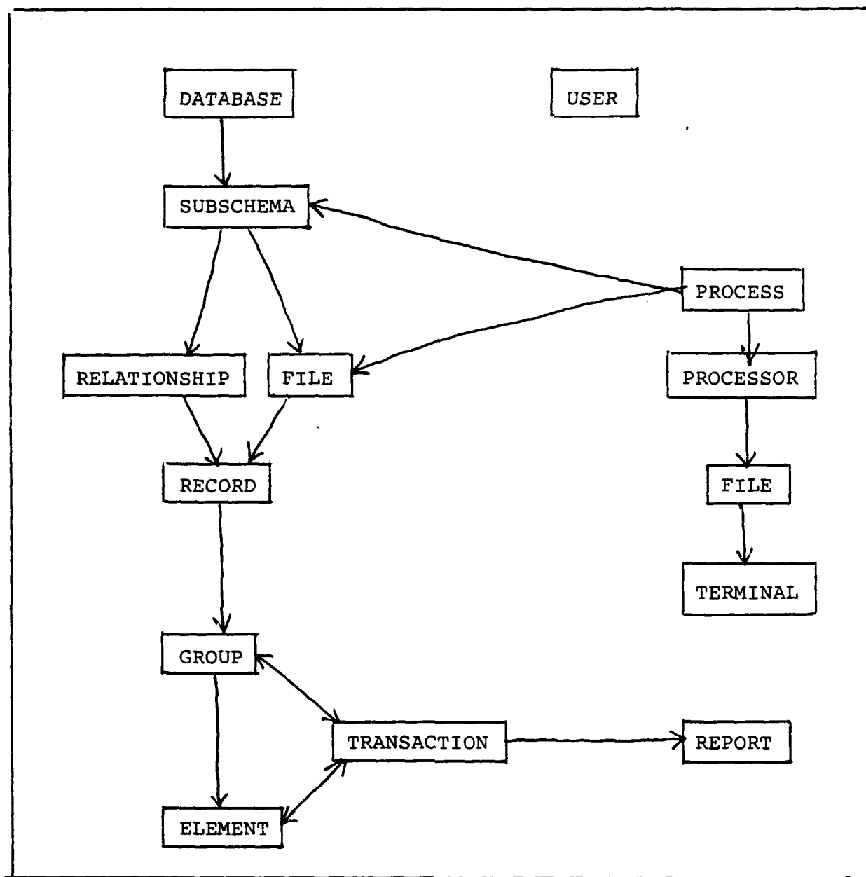
Figure 9--Logical Structure of a Typical DDS [Ref. 24]
