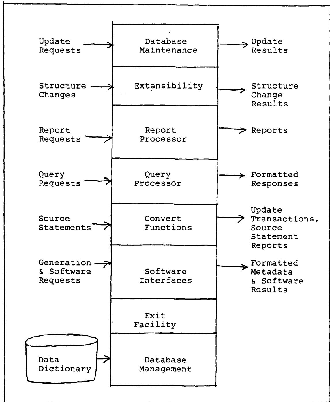
Figure 10--DDS Functions [Ref. 25]
