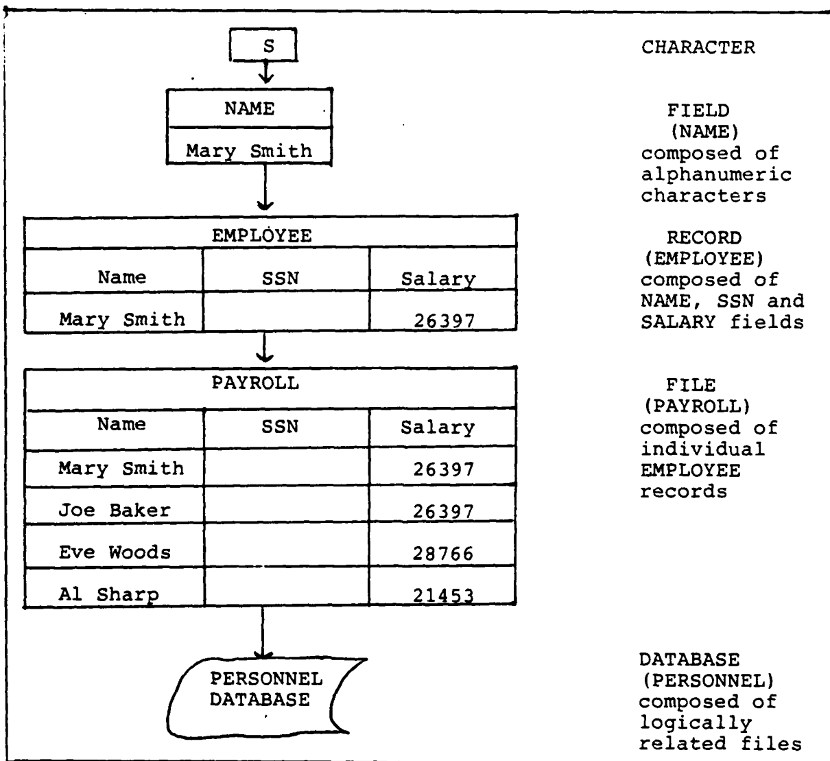
Figure 5--Hierarchy of Data Elements
