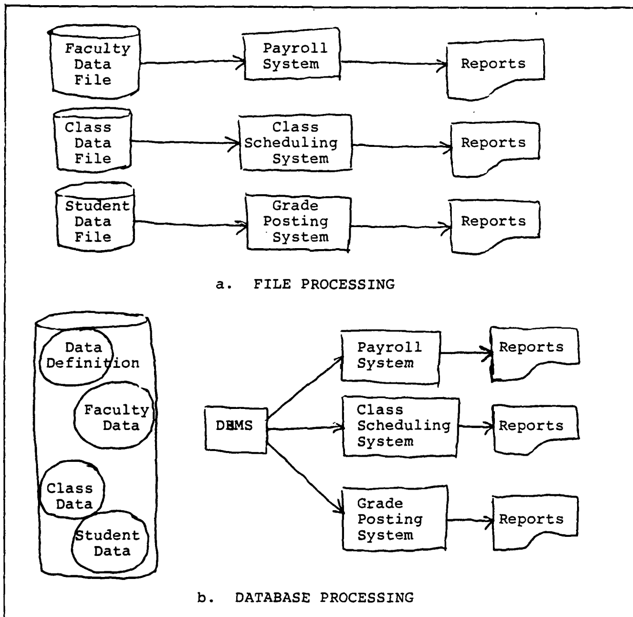
Figure 6--File/Database Processing [Ref. 6]
