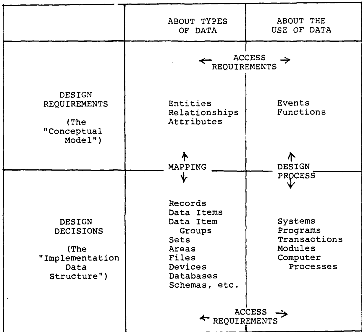
Figure 11--The Information in a Data Dictionary [Ref. 27]
