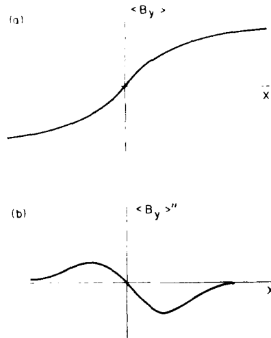
Fig. XI-1 — The initial profiles of \langle B_y \rangle and \langle B_y \rangle'' for a slab plasma unstable to tearing modes
