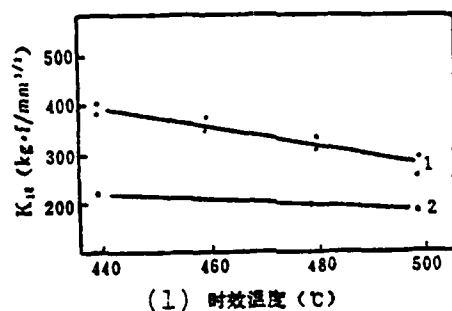
Fig. 1 The influences of different carbon contents on maraging steel K_{1C} : 1 - 0.01%C; 2 - 0.027%C.
