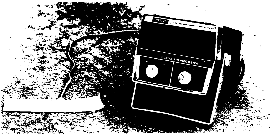
Figure 25. Typical setup for pavement temperature measurements
