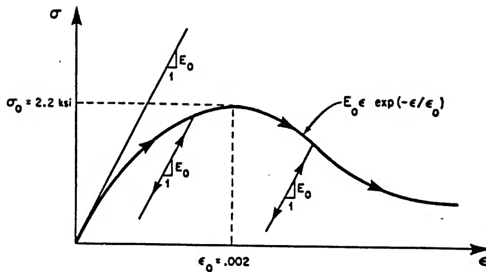
(a) Softening stress-strain model.
