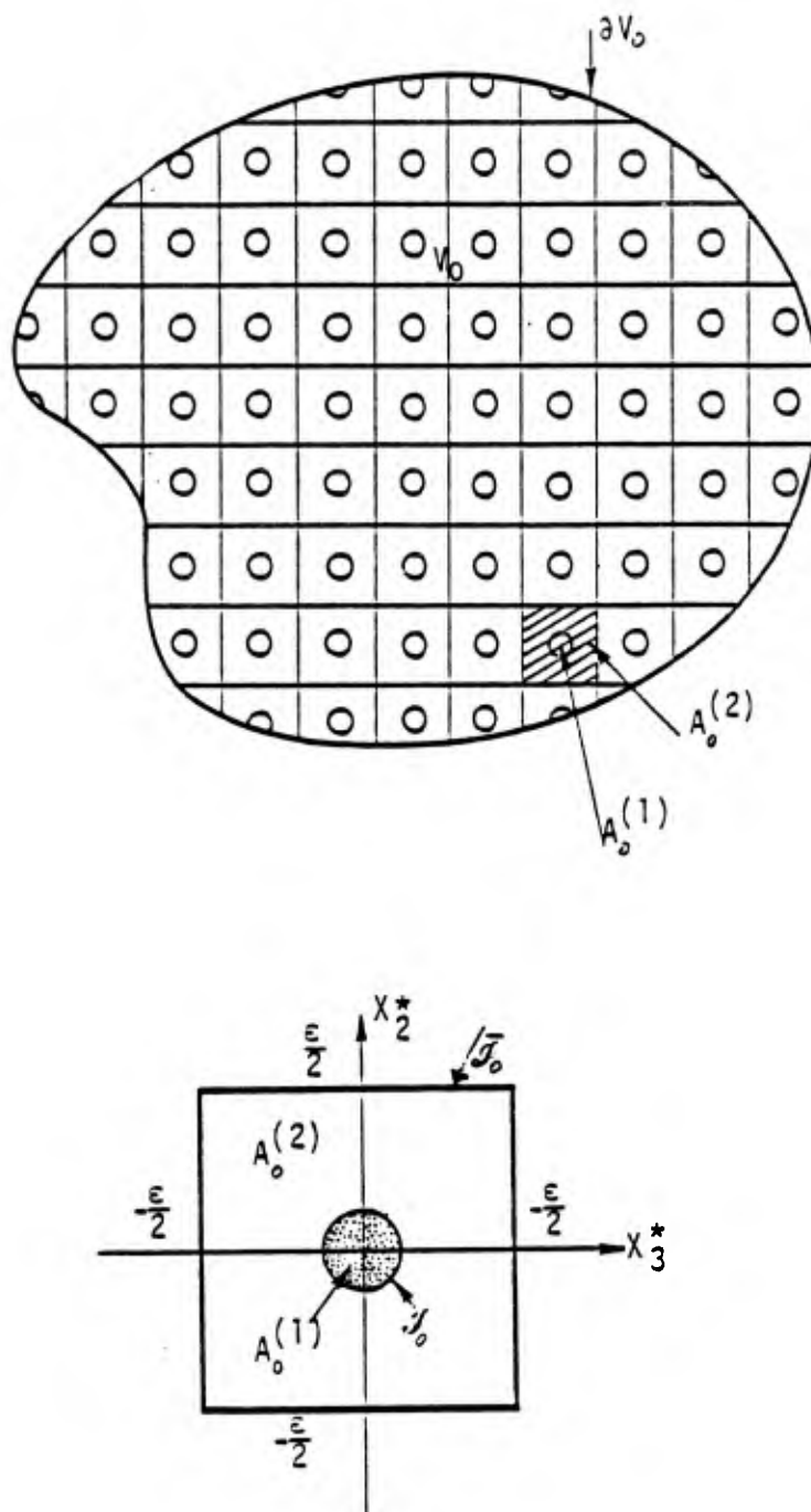
Figure 3.2. Cell geometry for densely reinforced concrete (shown in initial configuration).
