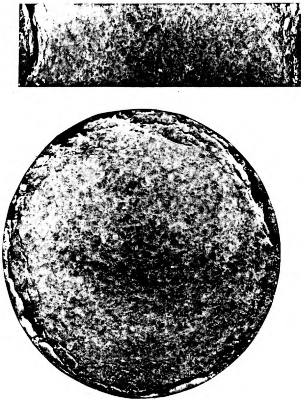
Figure 4.3. Cross-section and end view of 1/3:1 specimen (4-inch diameter) at advanced state of failure. (Georgia Cherokee marble) (From Reference 30).
