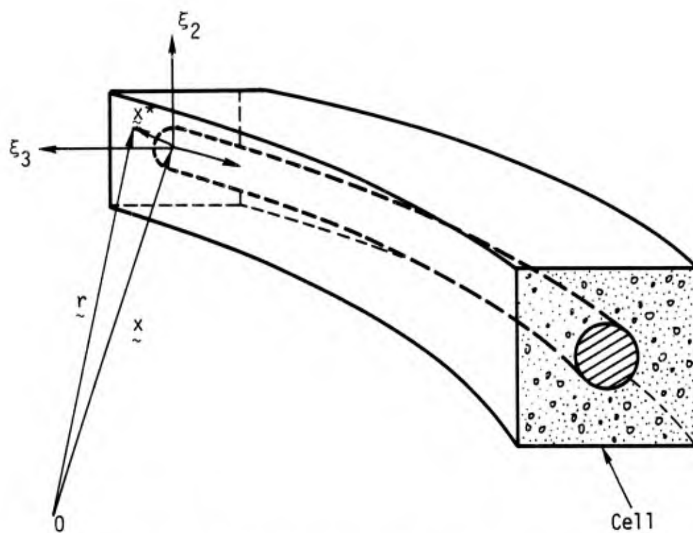
Figure 3.5(a). Geometry for sparse array.
