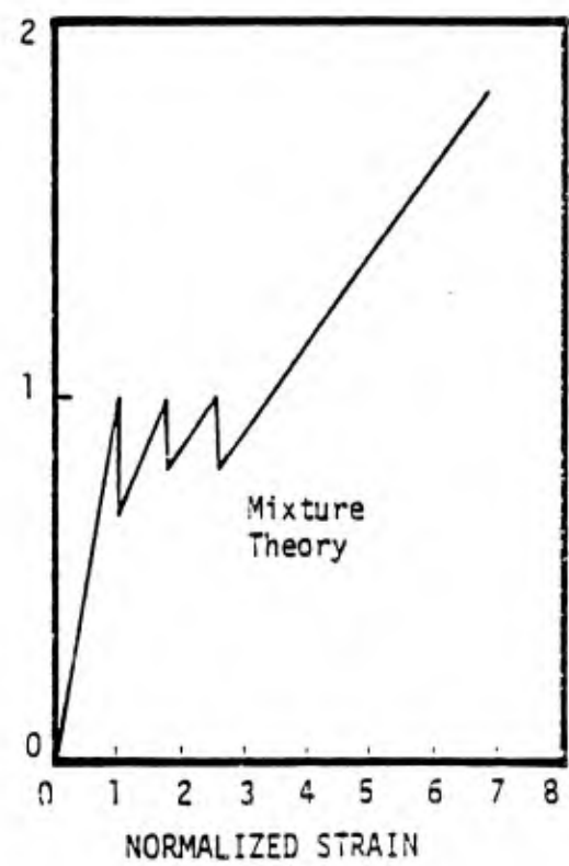
Figure 3.19. Comparisons of experiment and theory.
