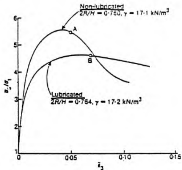
(a) Stress ratio versus axial strain.
