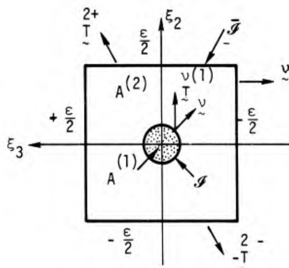
Figure 3.5(b). Cross-sectional geometry.
