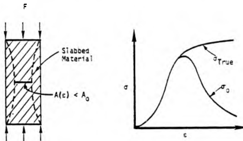
(a) Specimens with small L/D ratios.
