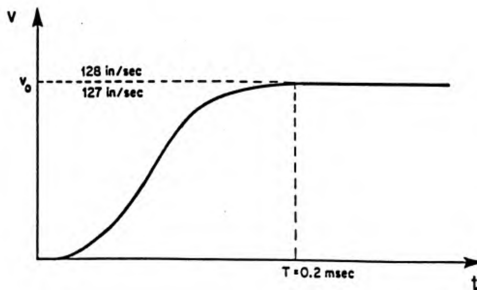
(b) Input boundary velocity history at x = 0 .
