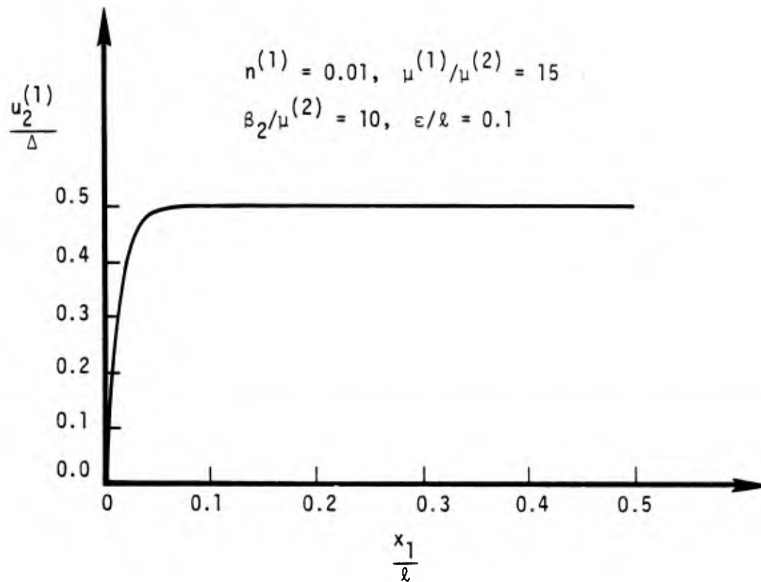
Figure 3.28. Displacement profile of steel.
