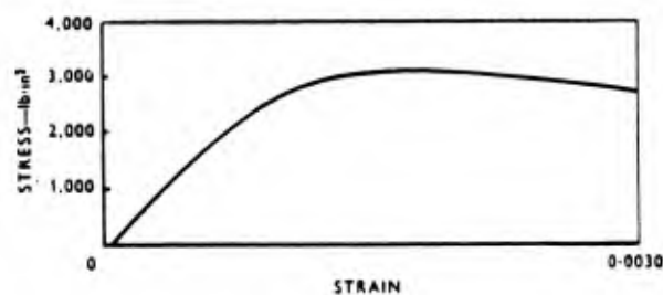
(b) Specimen 111 W 3-30 Strain: 0.0030
