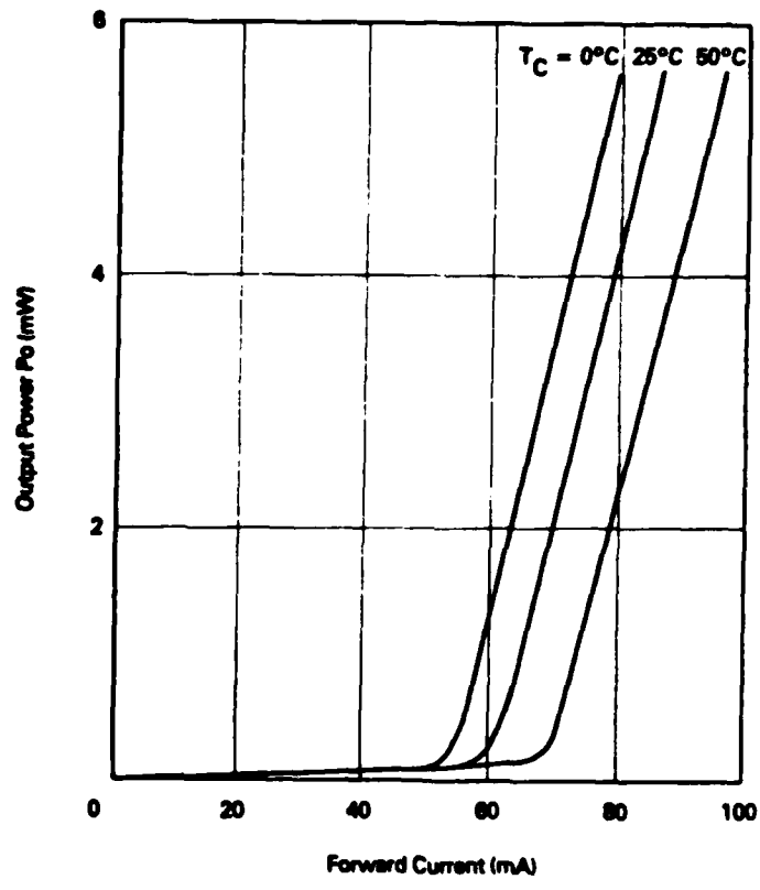
Figure 6. Output power versus forward current.
