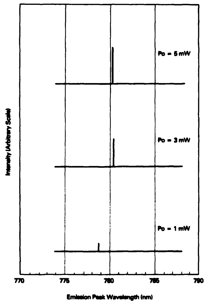
Figure 7. Output power dependence on emission spectra.
