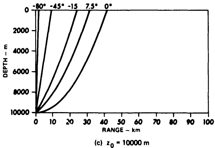
FIGURE 8 NORTH PACIFIC RAY PATHS
