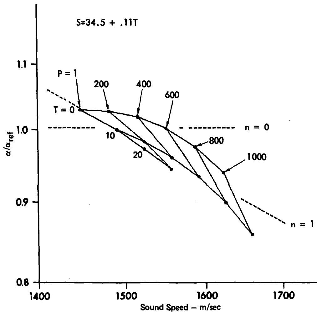
FIGURE C-3 \alpha/\alpha_{ref} versus c (LOG-LOG SCALES), FOR SEAWATER WITH SALINITY S = 34.5 + 0.11 T^{\circ}\text{oo}
