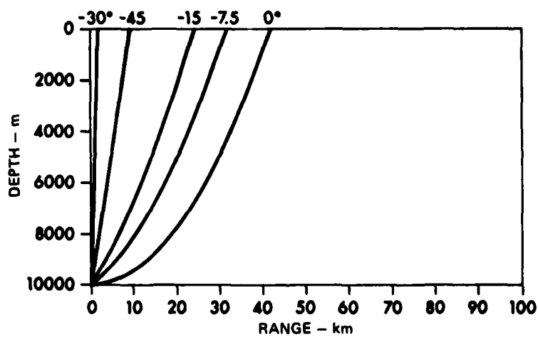
FIGURE 7 NORTH ATLANTIC RAY PATHS
