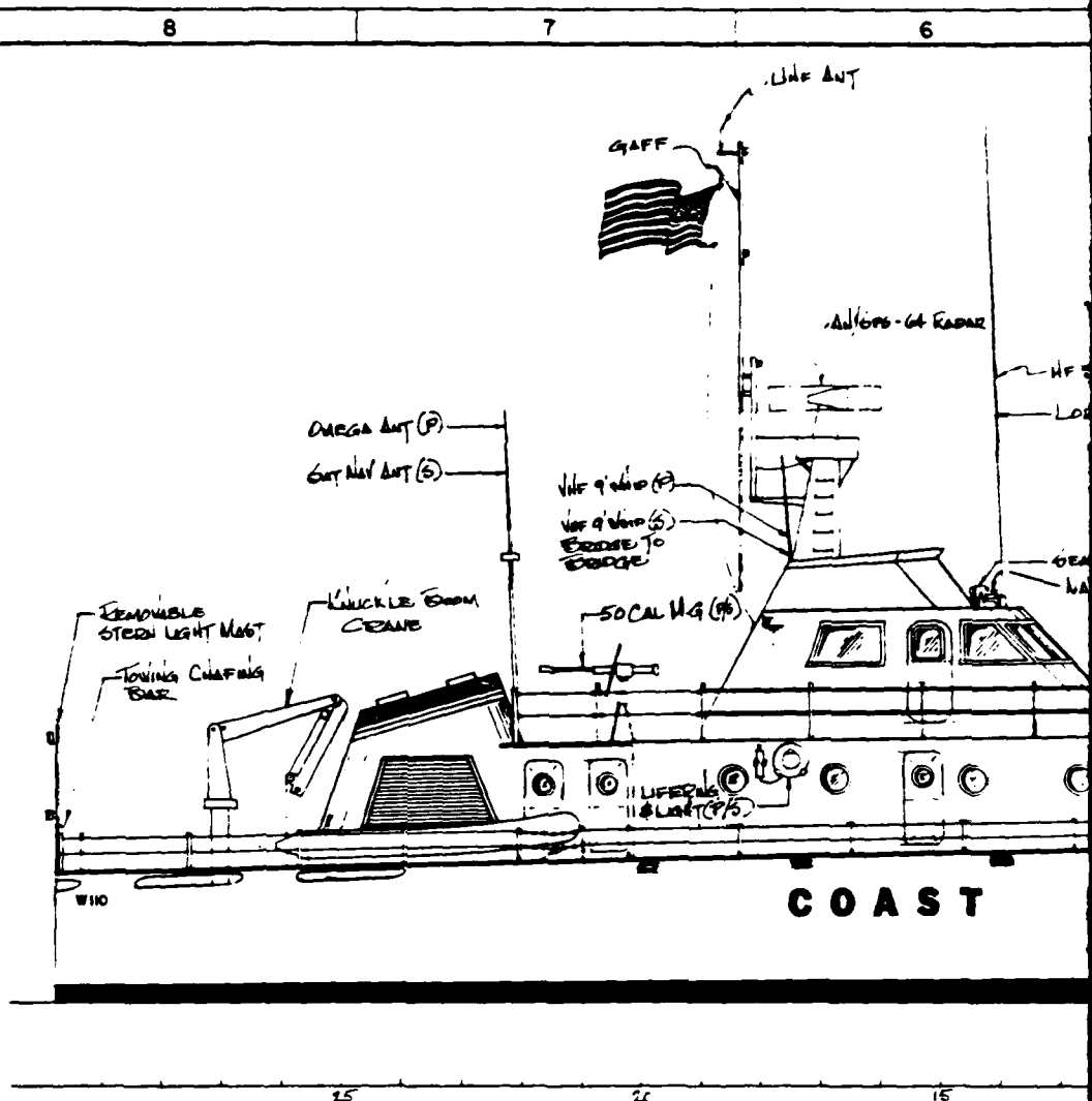
OUTBOARD PROFILE SCALE: 1/4" = 1'-0"
