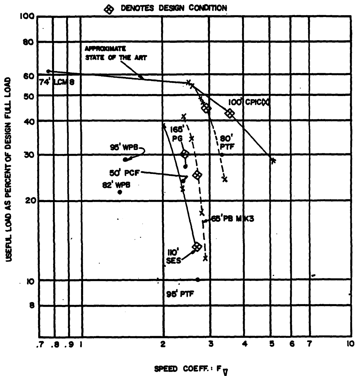
Figure A-2. Useful Load Fraction, State-of-the-Art
