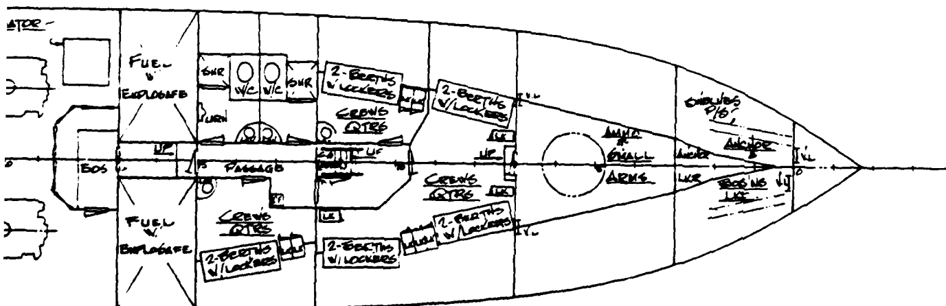
PLATFORM ARRANGEMENT PLAN
