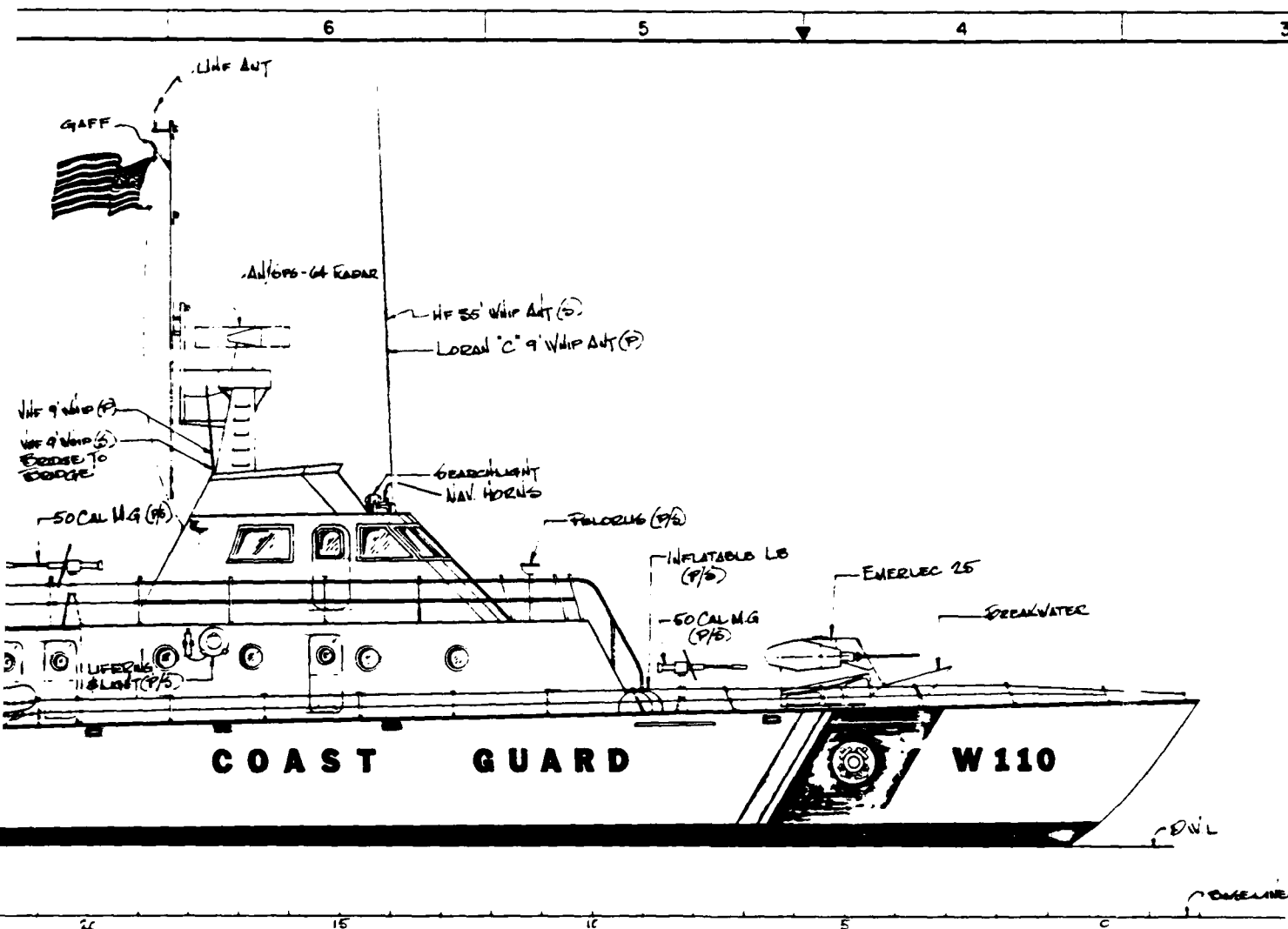
OUTBOARD PROFILE SCALE: \frac{1}{4} " = 1'-0"
