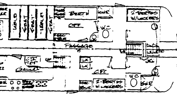
01 LEVEL ARRANGEMENT PLAN
