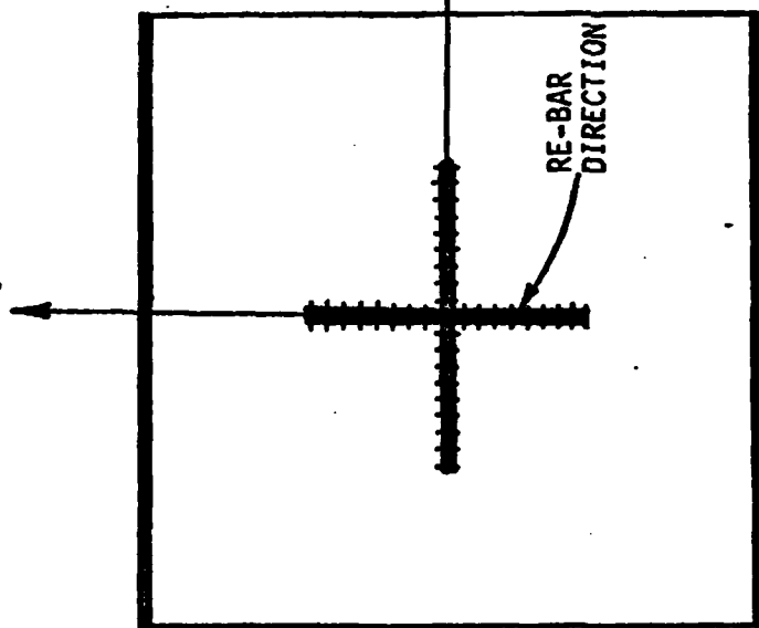
(a) EXAMPLE 1 STEEL COINCIDES WITH PRINCIPAL MOMENTS
