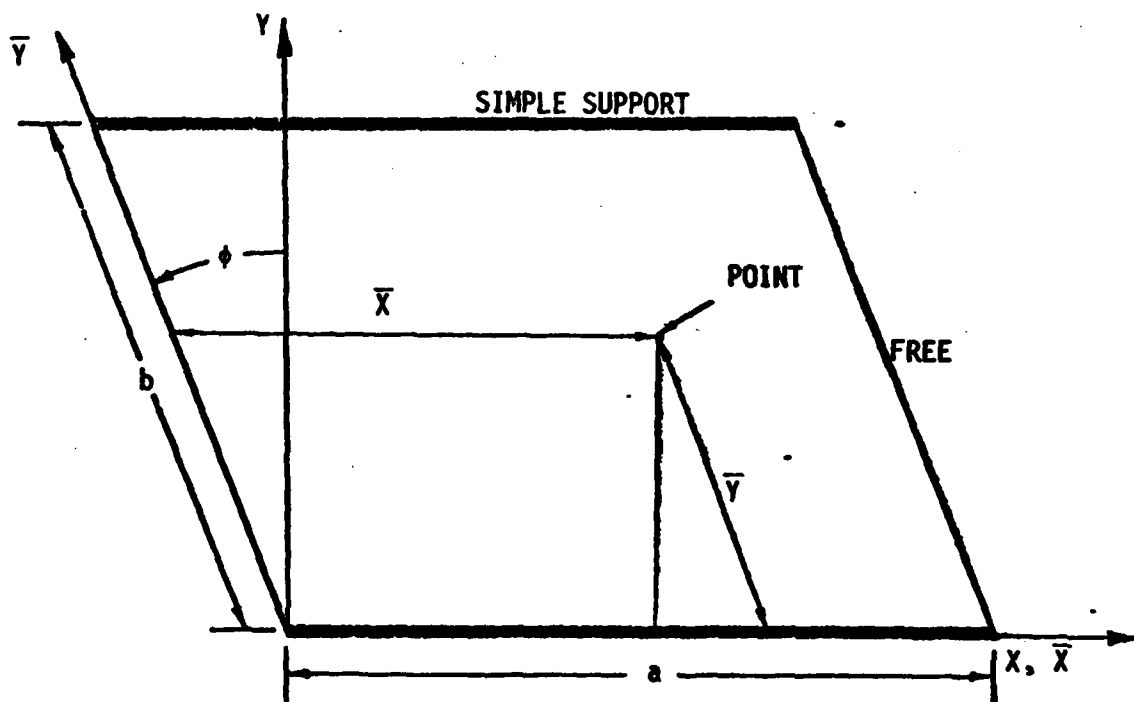
(b) SKEWED DECK
