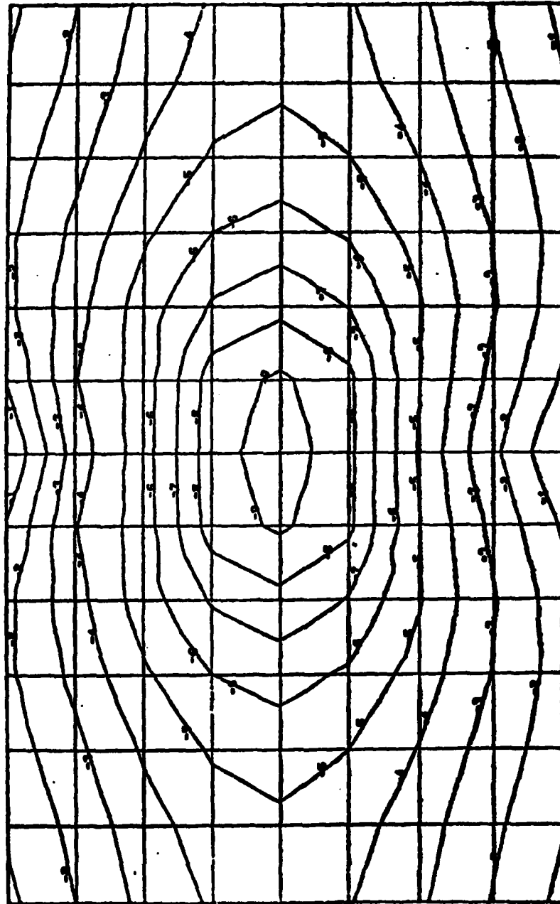
FIGURE C.3 CONTOUR: MAJOR PRINCIPAL MOMENT FOR PEAK SU-4 CENTER LOAD, SKEW = 0°
