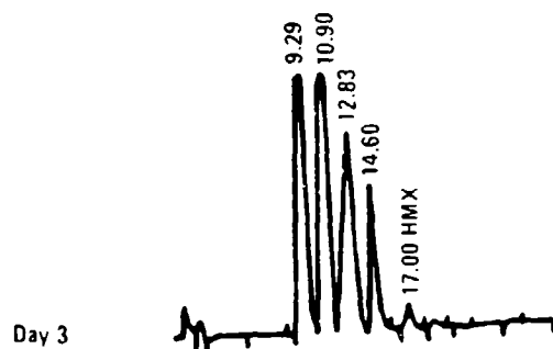
FIGURE 7 HPLC PROFILE OF HMX METABOLITES ON DAYS 1, 2, AND 3 Waters Radial Pak-A C 18 cartridge; Solvent: 20-40% B in A, where A is water and B is methanol acetonitrile (50-50) in 20-min linear gradient; Flow: 2 ml/min; Detection: UV @ 230 nm
