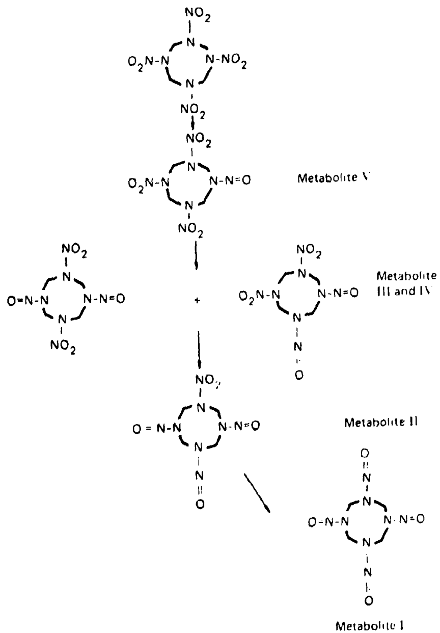
FIGURE 15 ANAEROBIC METABOLISM OF HMX
