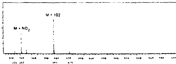
FIGURE 9 MASS SPECTRA FOR HMX
