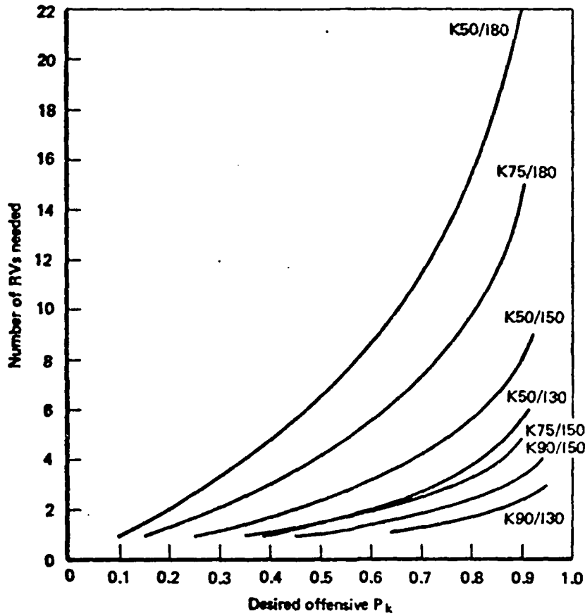
Fig. 1- Effect of ABM on point target coverage (K#/l# = offensive probability of kill/defensive probability of kill)
