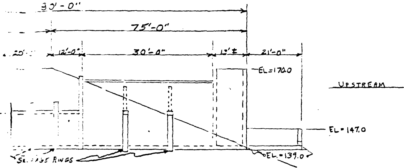
VATION (EAST) OF SPILLWAY STRUCTURE SCALE = 1" = 20'-0"
