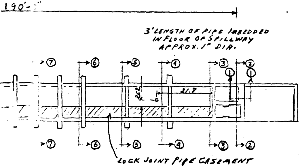
CF. SPILLWAY STRUCTURE SCALE = 1" = 20'-0"
